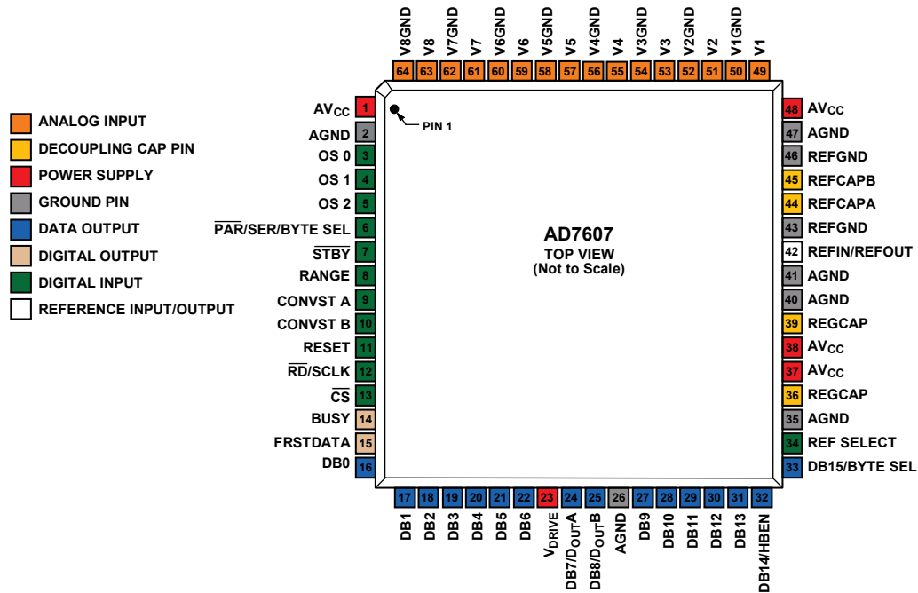
Figure 8. Pin Configuration
