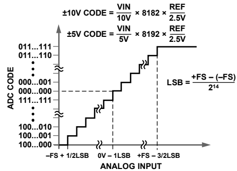
Figure 35. Transfer Characteristics
