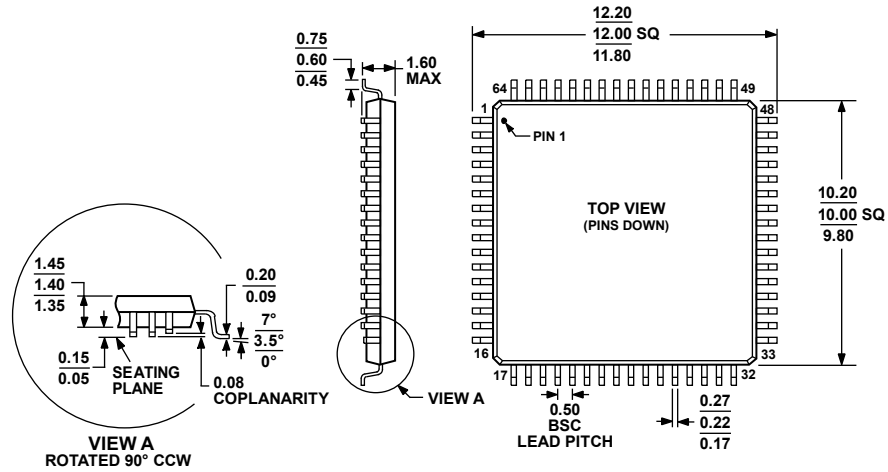
COMPLIANT TO JEDEC STANDARDS MS-026-BCD Figure 55. 64-Lead Low Profile Quad Flat Package [LQFP] (ST-64-2) Dimensions shown in millimeters
