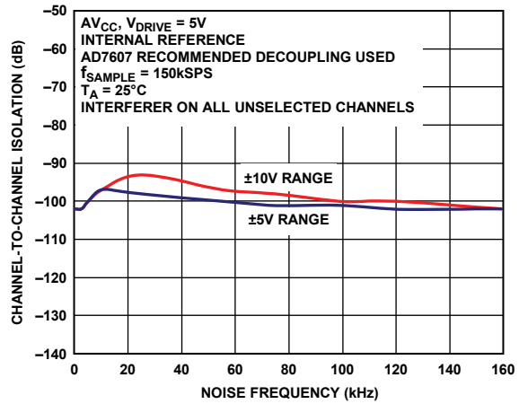
Figure 29. Channel-to-Channel Isolation
