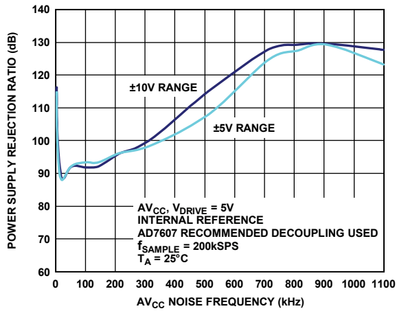
Figure 28. PSRR
