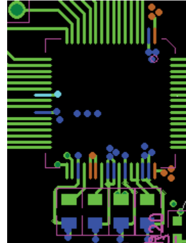
Figure 52. Top Layer Decoupling REF IN /REF OUT , REFC APA , REFC PB , and REGCAP Pins
