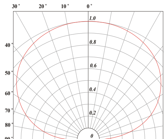
Radiation Pattern
