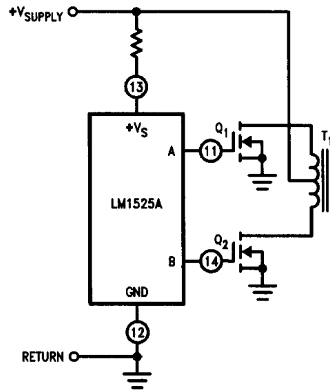
3 MOSFET Drive for Push-Pull Converters
