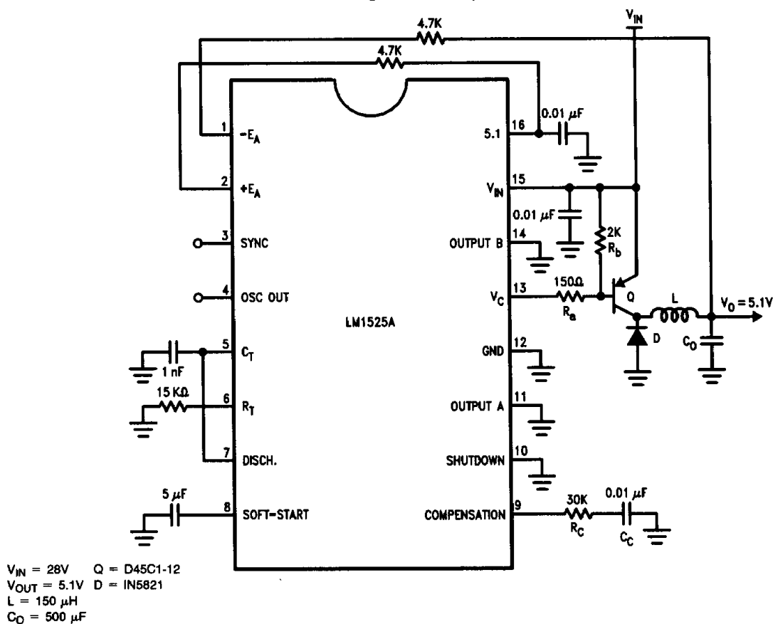
5 Watt Single Ended Step Down Converter
