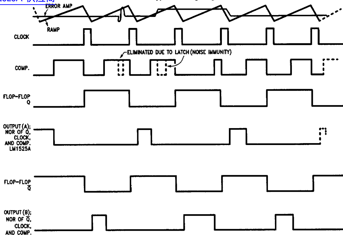
LM1525A Typical Timing Diagram
