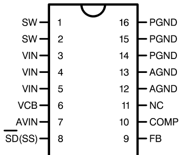
16-Lead TSSOP (MTC)
