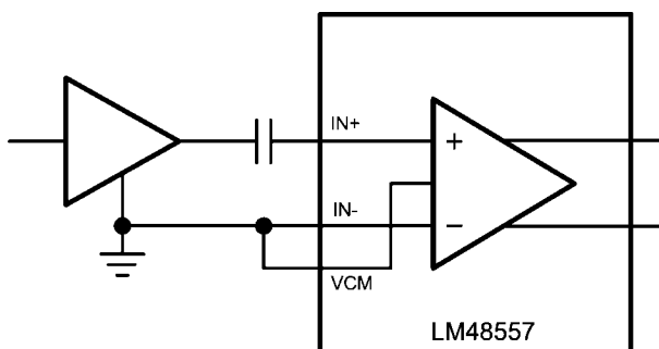
Non-Inverting Configuration
