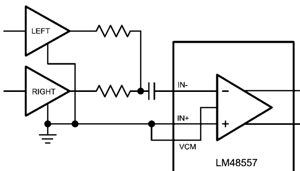
Inverting Configuration
