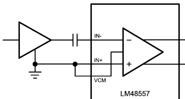
Inverting Configuration
