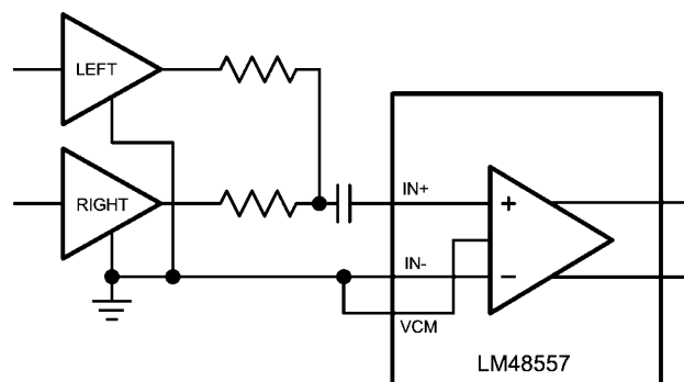
Non-Inverting Configuration
