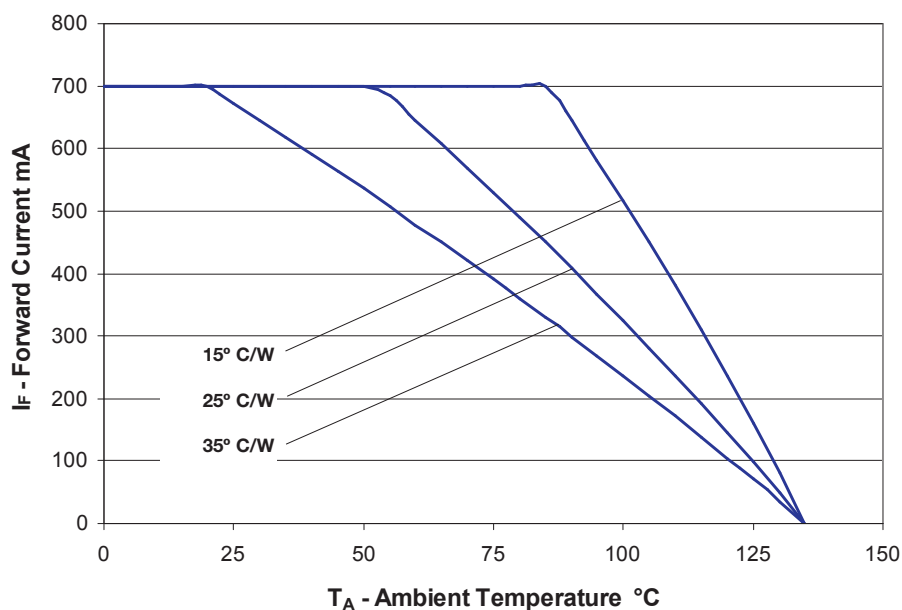
Figure 15: Maximum forward current vs. ambient temperature, based on T_{J\text{MAX}} = 135^{\circ}\text{C} .
