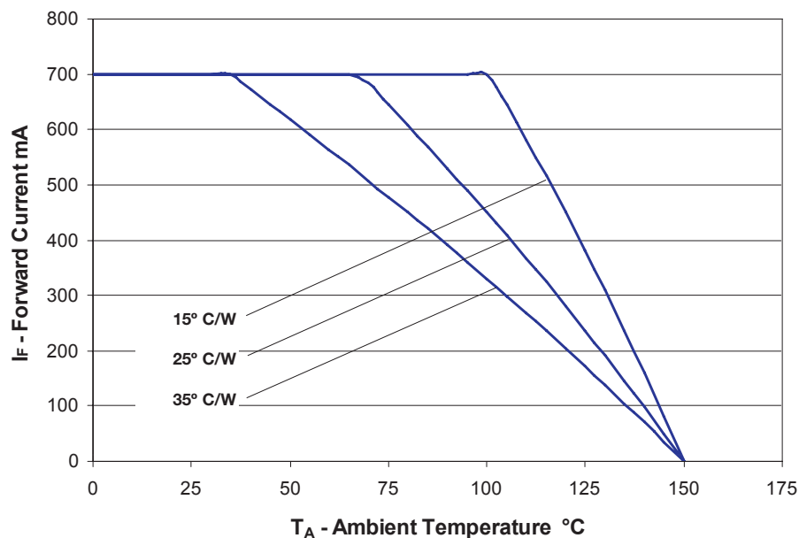
Figure 14: Maximum forward current vs. ambient temperature, based on T_{J\text{MAX}} = 150^{\circ}\text{C} .
