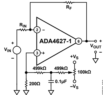
Figure 38. Alternate Offset Null Circuit for Inverting Stage
