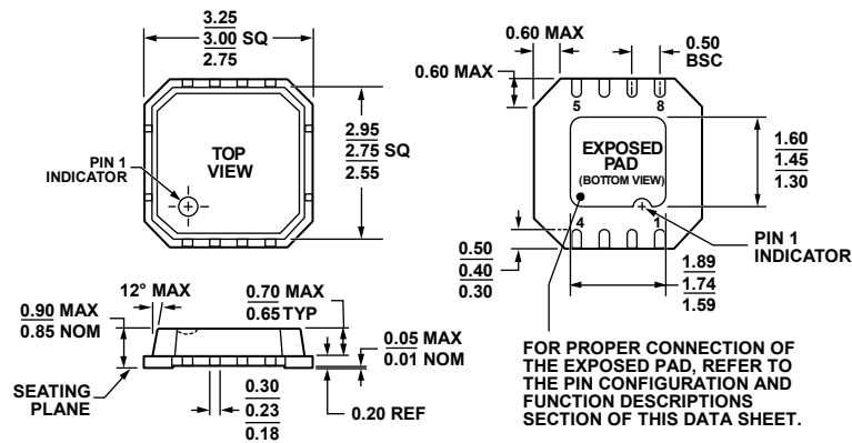
Figure 42. 8-Lead Lead Frame Chip Scale Package [LFCSP_VD]
