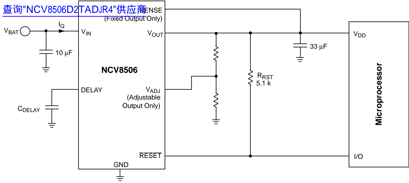
Figure 1. Application Diagram
