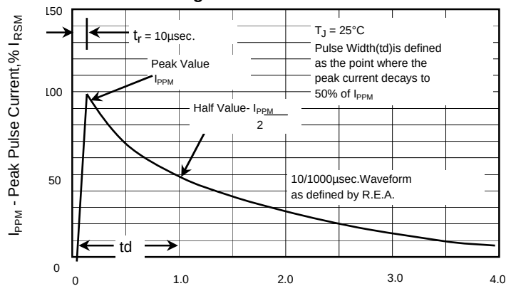
Fig.3 - Pulse Waveform
