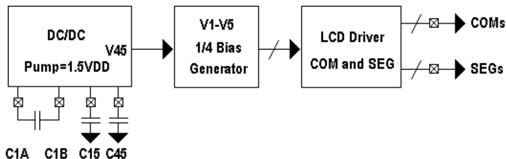
Fig.12 LCD DC/DC and Bias Generator
