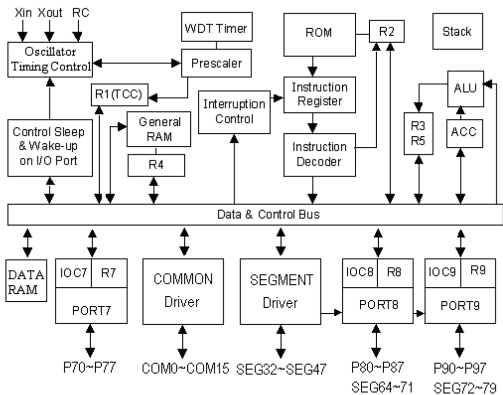
Fig. 2b System Functional Block Diagram
