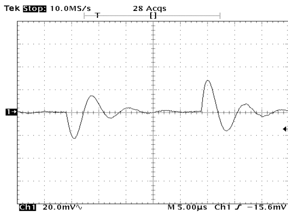
FIGURE 24. LINE TRANSIENT RESPONSE, 0.001μF LOAD CAPACITANCE
