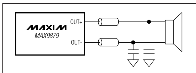
Figure 13. Optional Ferrite Bead Filter
