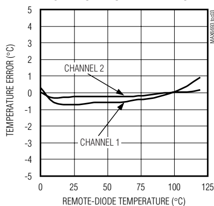
REMOTE-DIODE TEMPERATURE ERROR vs. REMOTE-DIODE TEMPERATURE
