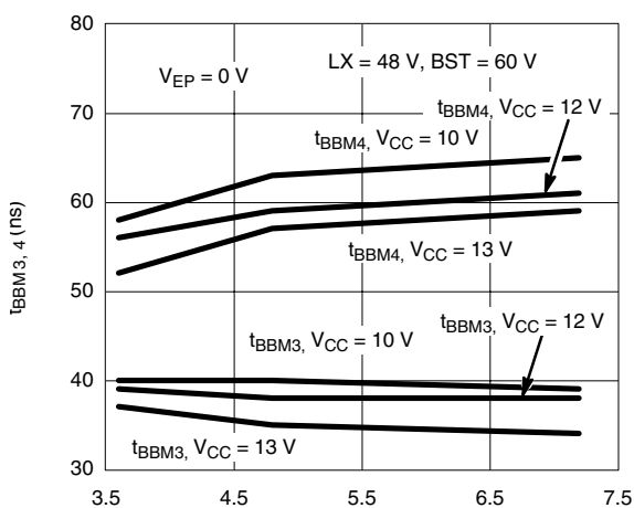
t_{BBM3,4} vs. V_{CC} vs. V_{INDET} , f_{OSC} < 200\text{ kHz}
