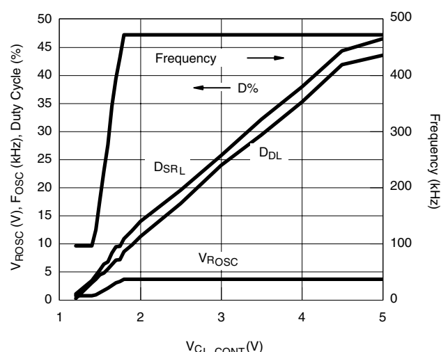
V_{ROSC} , F_{osc} , and Duty Cycle vs. V_{CL\_CONT}
