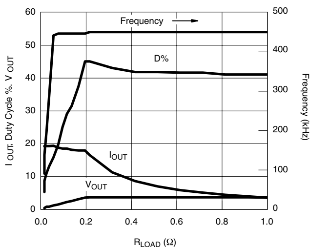
I_{OUT} vs. R_{LOAD} ( V_{IN} = 72\text{ V} )
