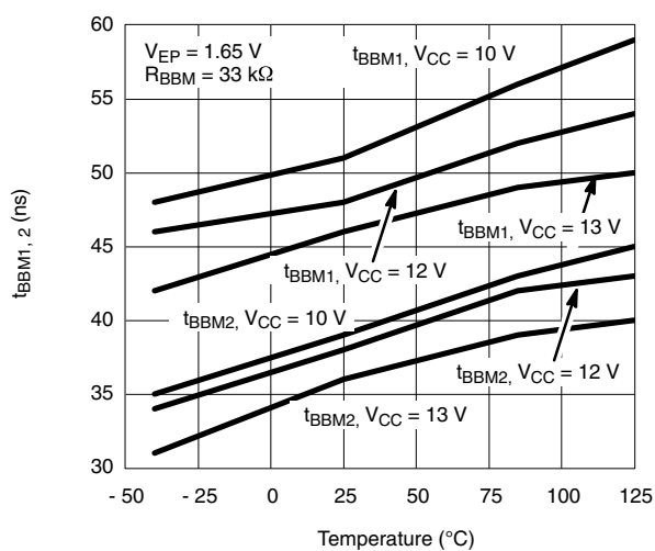
t_{BBM1,2} vs. Temperature, V_{EP} = 1.65 V
