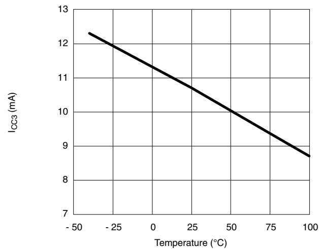
I_{CC3} vs. Temperature V_{CC} = 12\text{ V}
