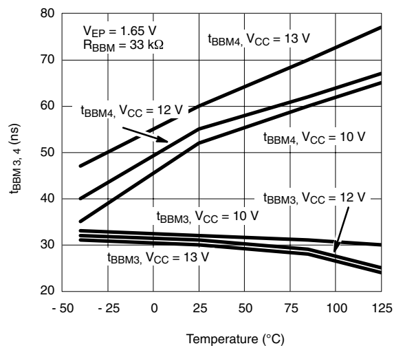
t_{BBM3,4} vs. Temperature, V_{EP} = 1.65 V
