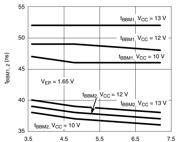
t_{BBM1,2} vs. V_{CC} vs. V_{INDET}
