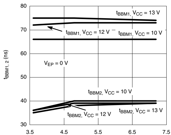
t_{BBM1,2} vs. V_{CC} vs. V_{INDET} , f_{OSC} < 200\text{ kHz}
