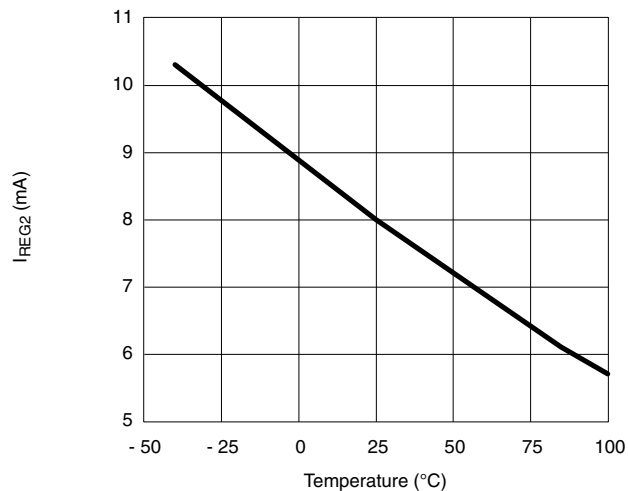
I_{REG2} vs. Temperature, V_{CC} = 12\text{ V}
