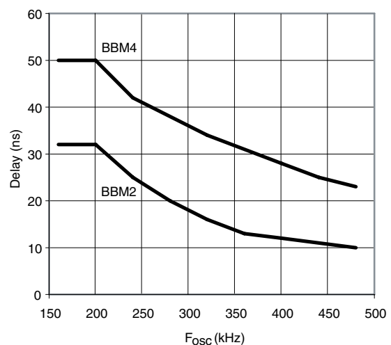
Figure 9. Reduction in BBM2 and BBM4 Si9122E BBM vs. F_{osc} ; V_{IN} = 50 V, V_{CC} = 10 V, BST = 60 V, LX = 50 V, V_{EP} = 0 V
