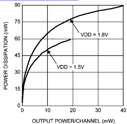
Power Dissipation vs Output Power R_L = 32\Omega , f = 1\text{kHz}
