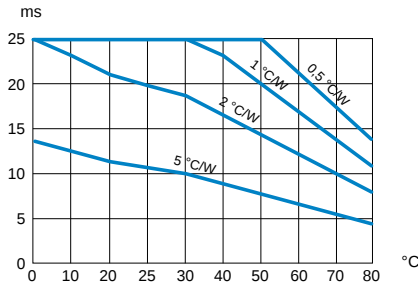
Thermal curves
