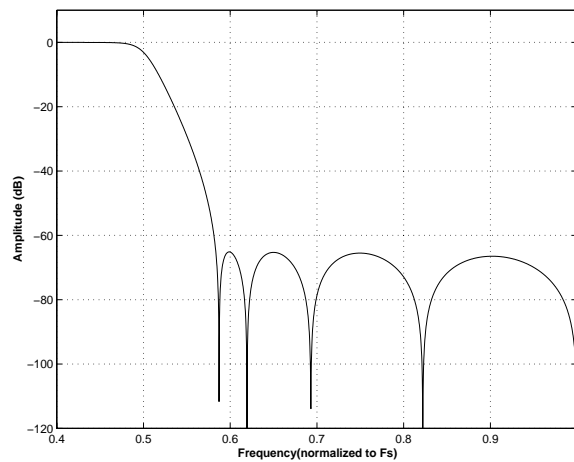
Figure 17. Single-Speed (slow) Stopband Rejection
