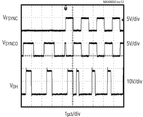
SYNCHRONIZATION WAVEFORMS
