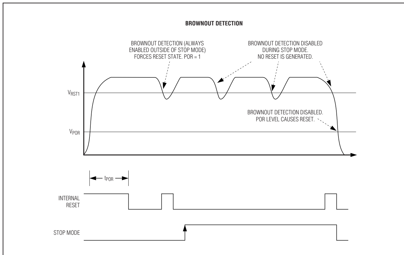
Figure 3. Brownout Reset
