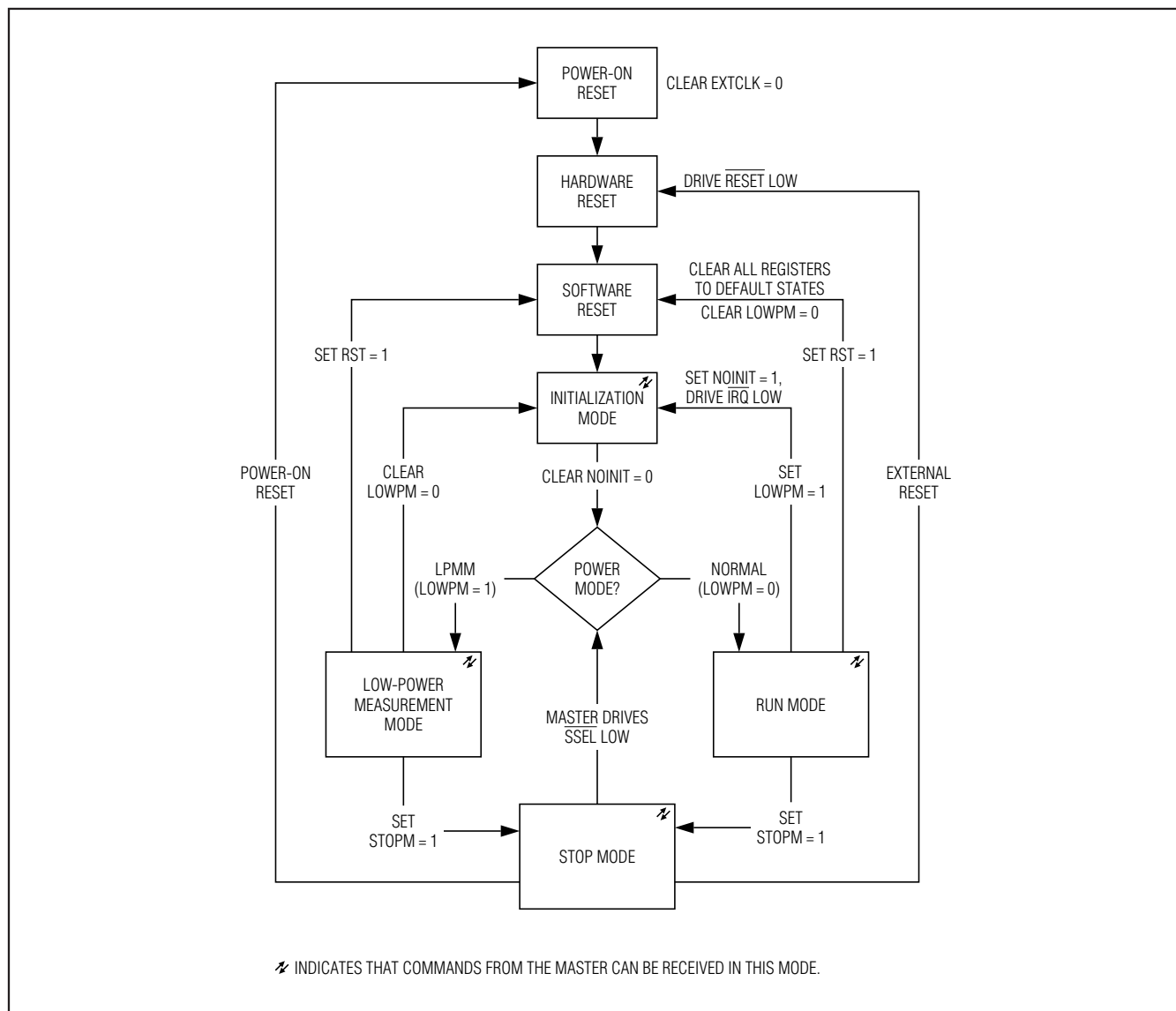
Figure 1. Operating Modes
