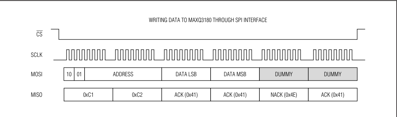
Figure 7. Write SPI Transfer
