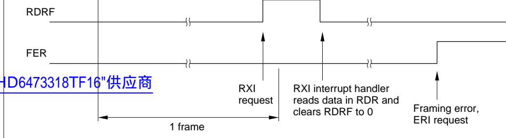
Figure 14.8 Example of SCI Receive Operation (8-Bit Data with Parity and One Stop Bit)
