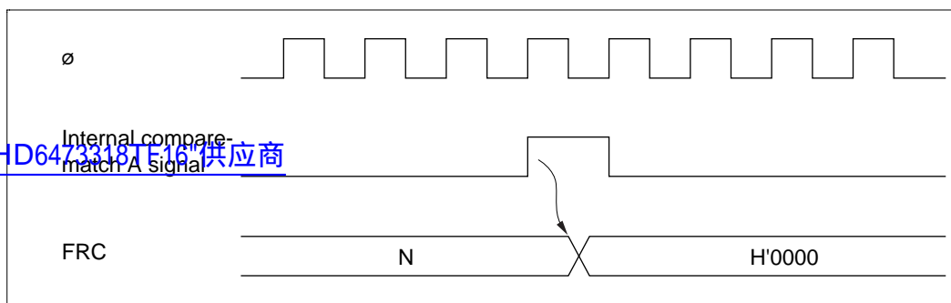
Figure 9.7 Clearing of FRC by Compare-Match A
