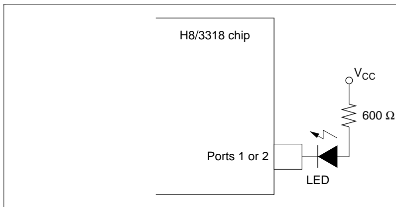
Figure 19.2 Example of Circuit for Driving an LED
