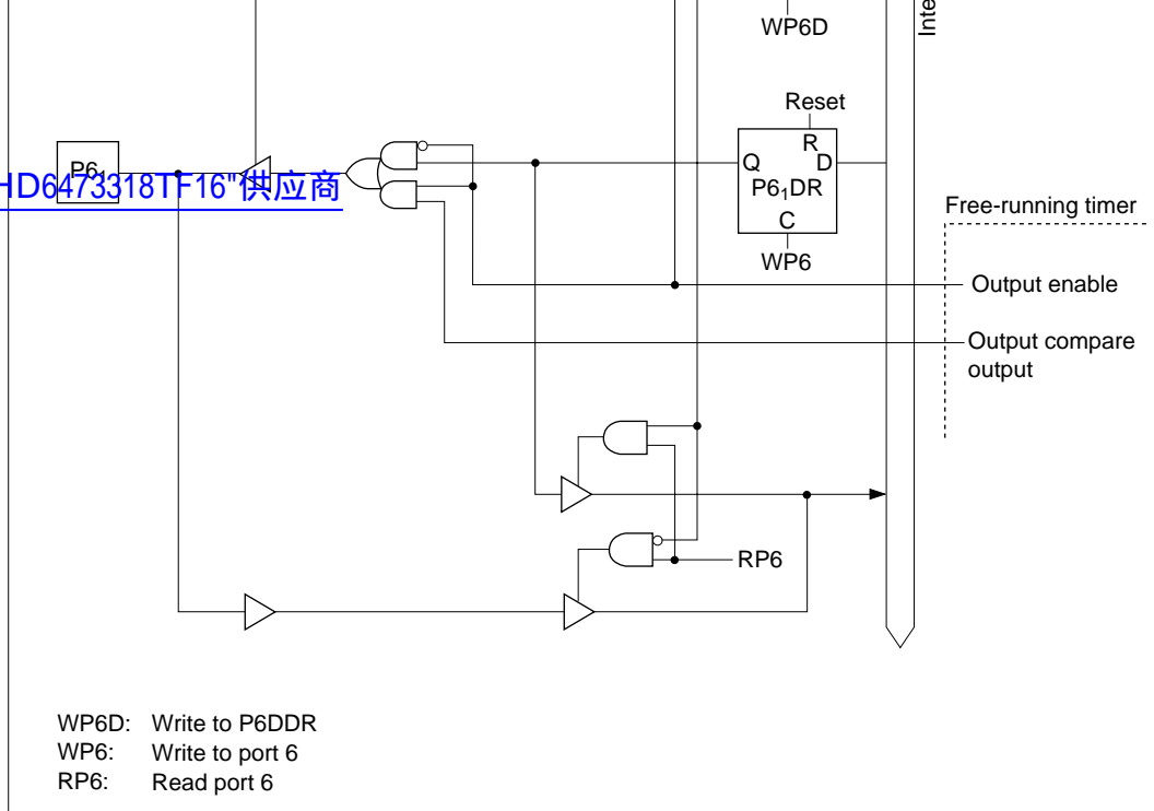
Figure C.6 (b) Port 6 Block Diagram (Pin P6I)
