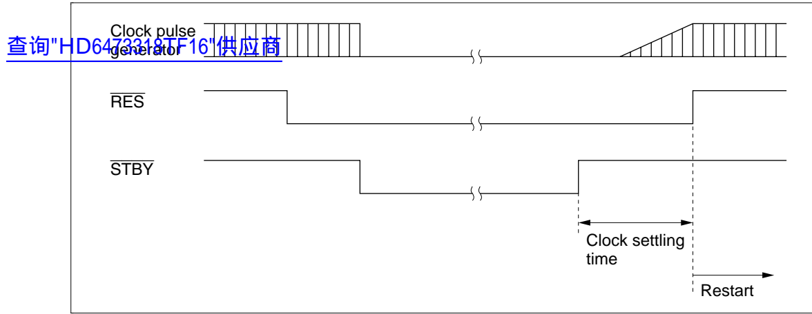
Figure 18.2 Hardware Standby Mode Timing
