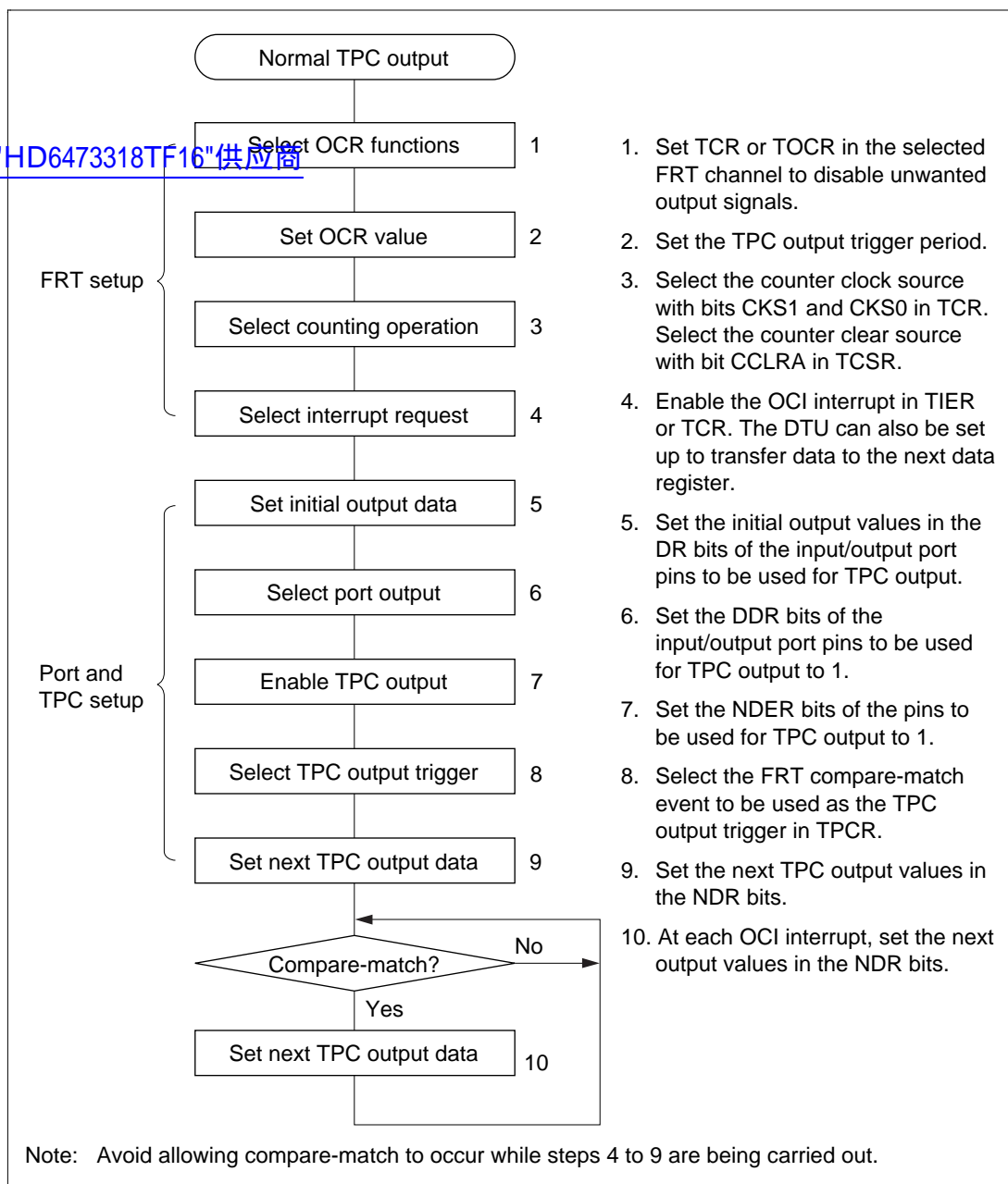
Figure 12.4 Setup Procedure for Normal TPC Output (Example)
