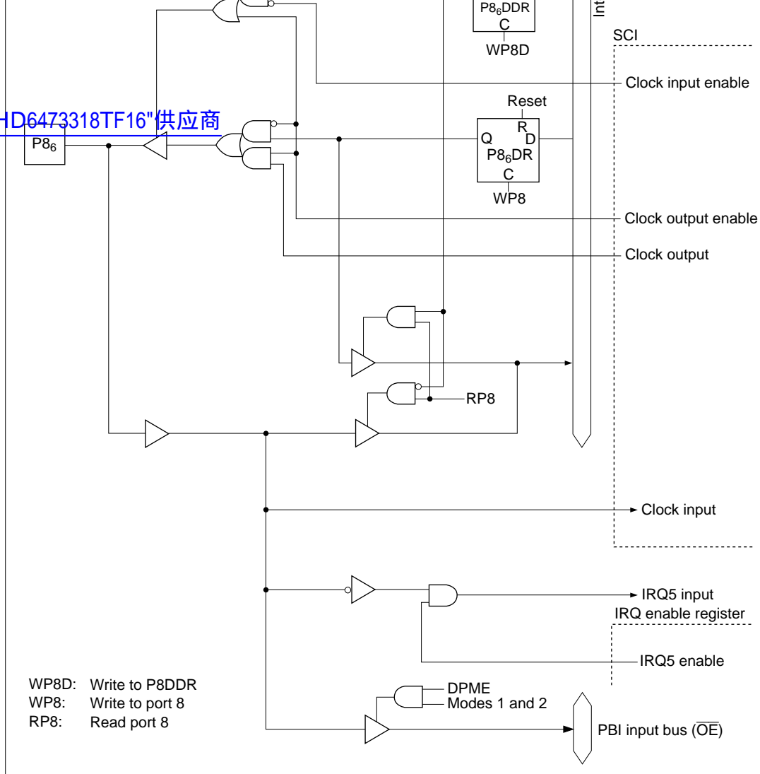
Figure C.8 (e) Port 8 Block Diagram (Pin P8 6 )
