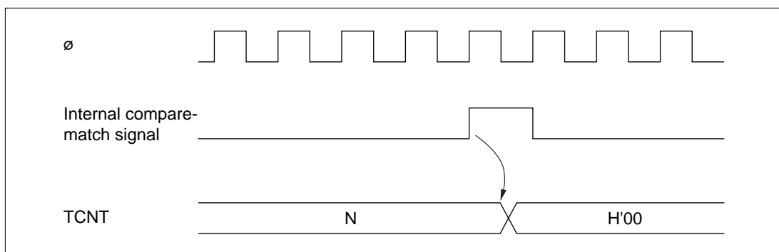
Figure 11.6 Timing of Compare-Match Clear
