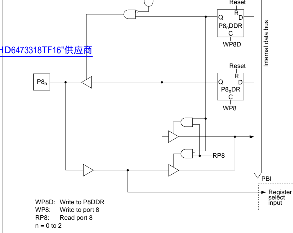
Figure C.8 (a) Port 8 Block Diagram (Pins P8 0 to P8 2 )
