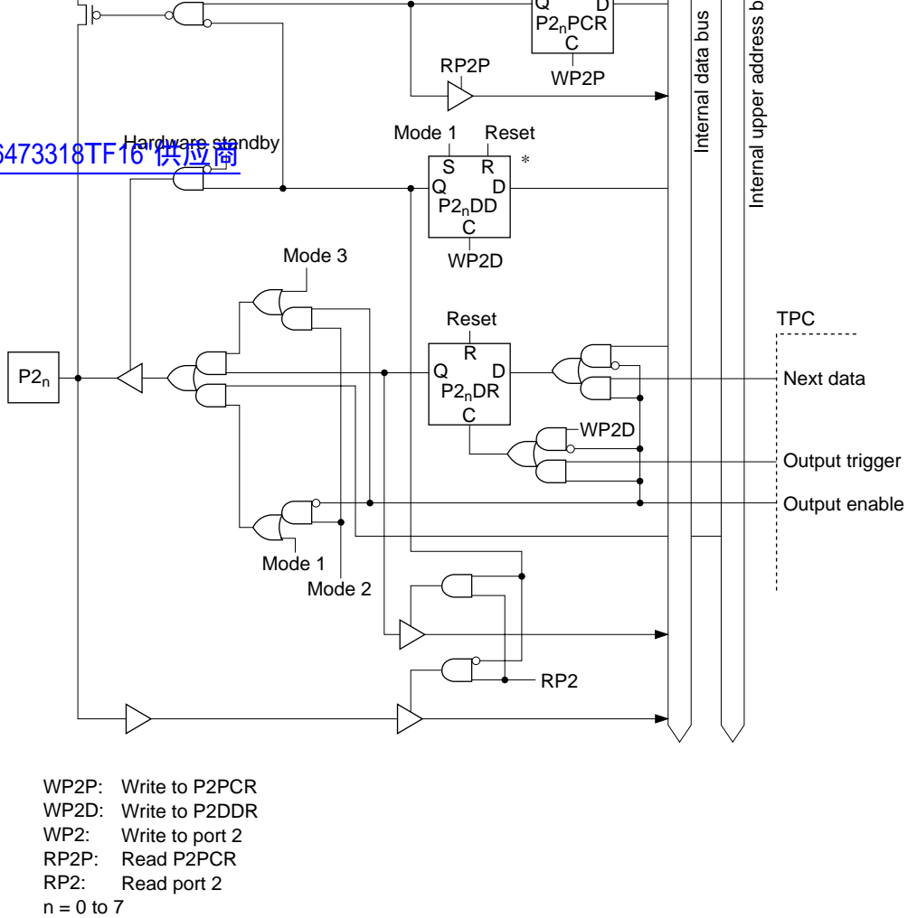
Figure C.2 Port 2 Block Diagram
