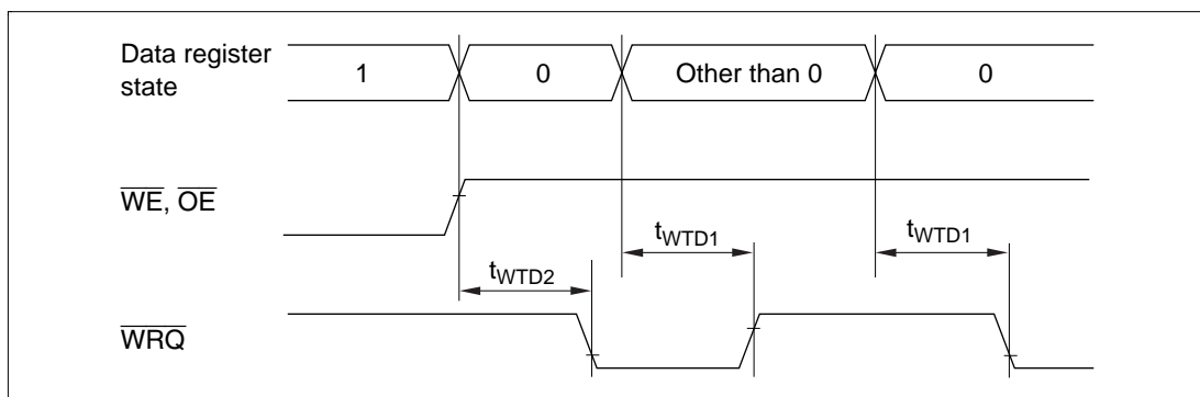
Figure 19.21 \overline{\text{WRQ}} Output Timing
