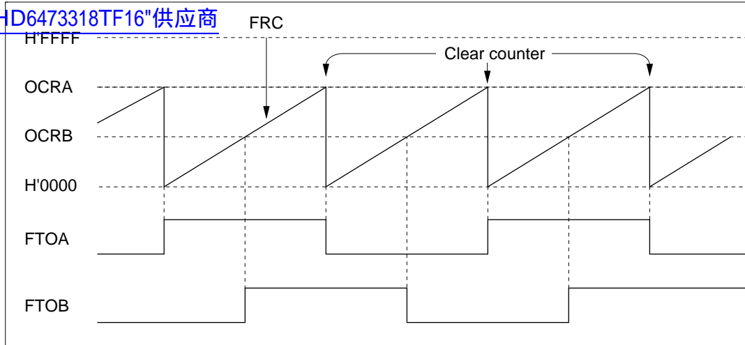
Figure 9.15 Square-Wave Output (Example)
