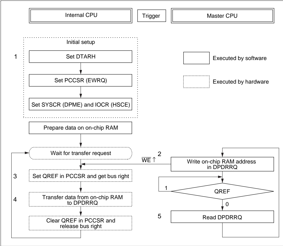
Figure 5.15 Flowchart of Buffer Query in DPRAM Mode
