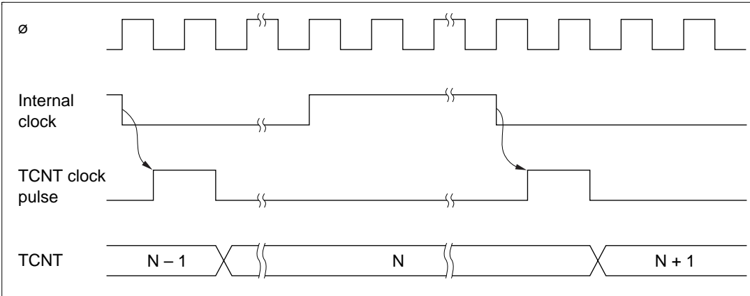
Figure 11.2 Count Timing for Internal Clock Input
