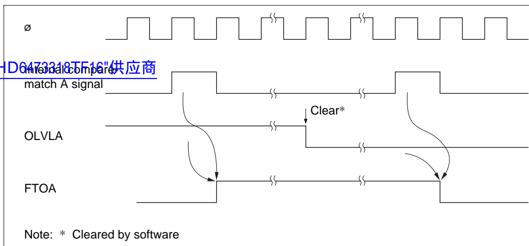
Figure 10.5 Timing of Output Compare A
