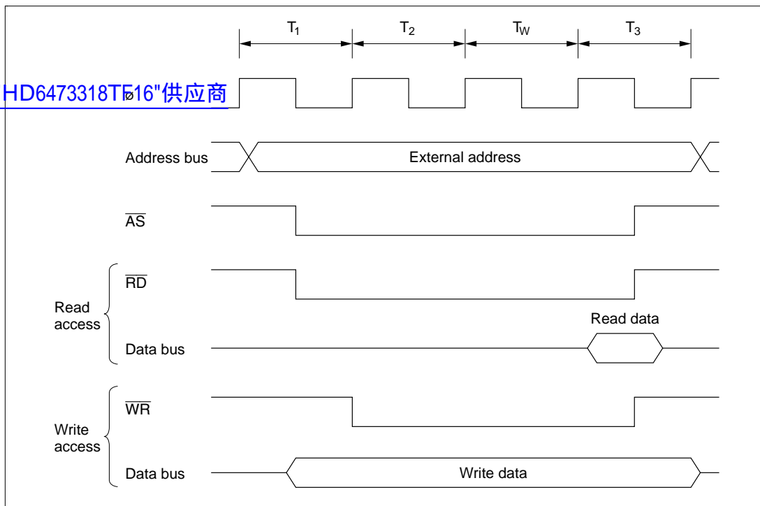
Figure 6.2 Programmable Wait Mode
