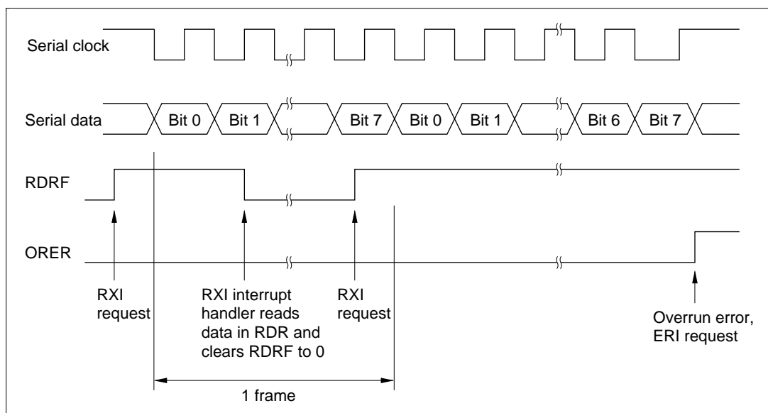
Figure 14.16 Example of SCI Receive Operation
