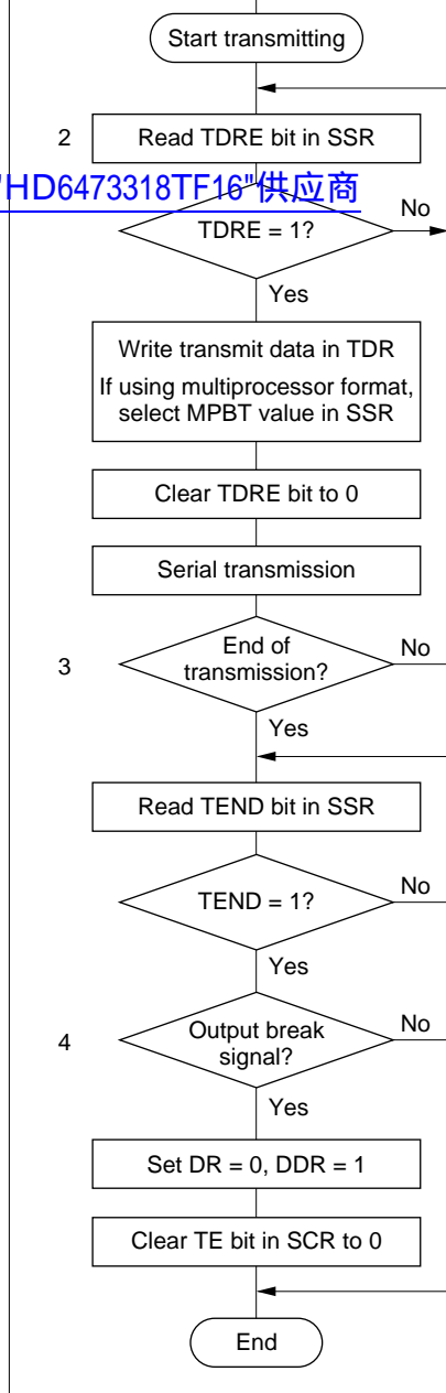
Figure 14.5 Sample Flowchart for Transmitting Serial Data
