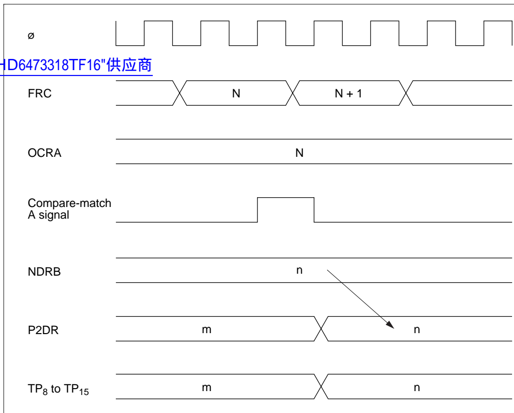
Figure 12.3 Timing of Transfer of Next Data Register Contents and Output (Example)
