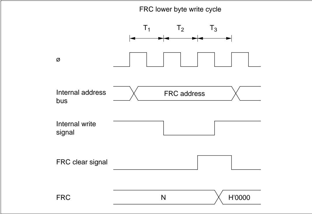
Figure 10.12 FRC Write-Clear Contention
