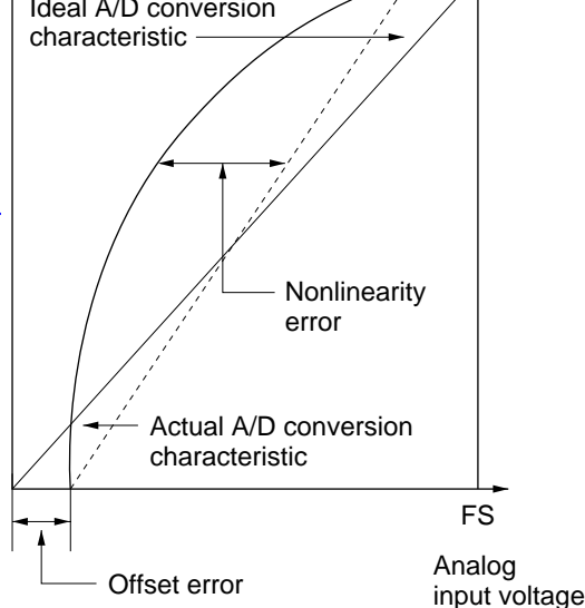
Figure 15.9 A/D Conversion Precision Definitions (2)
