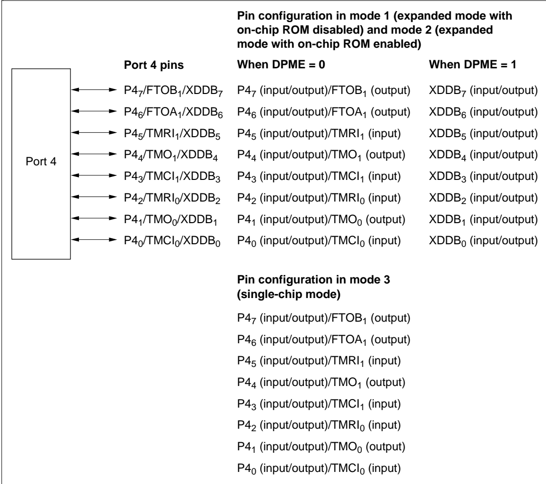
Figure 8.12 Port 4 Pin Configuration
