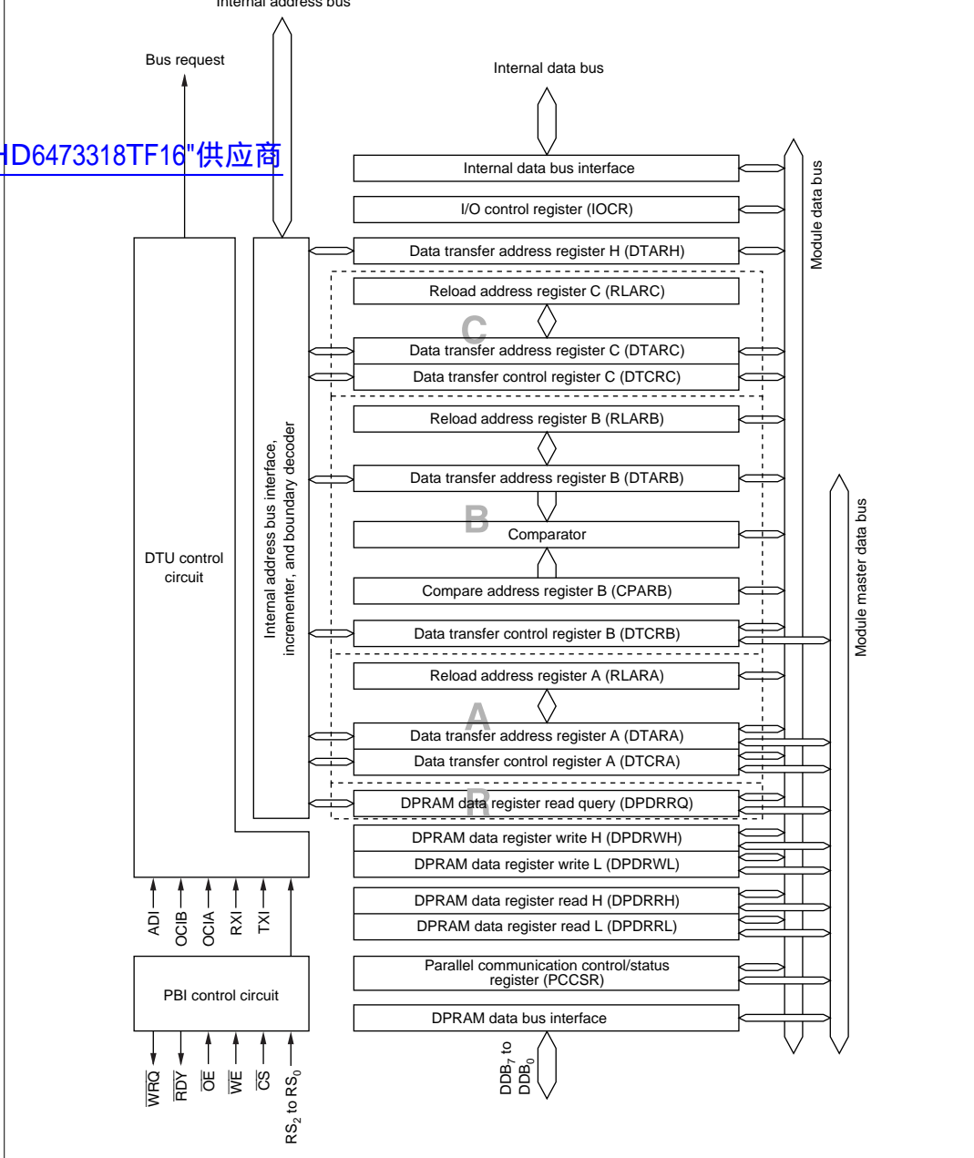
Figure 5.6 DTU and PBI Block Diagram
