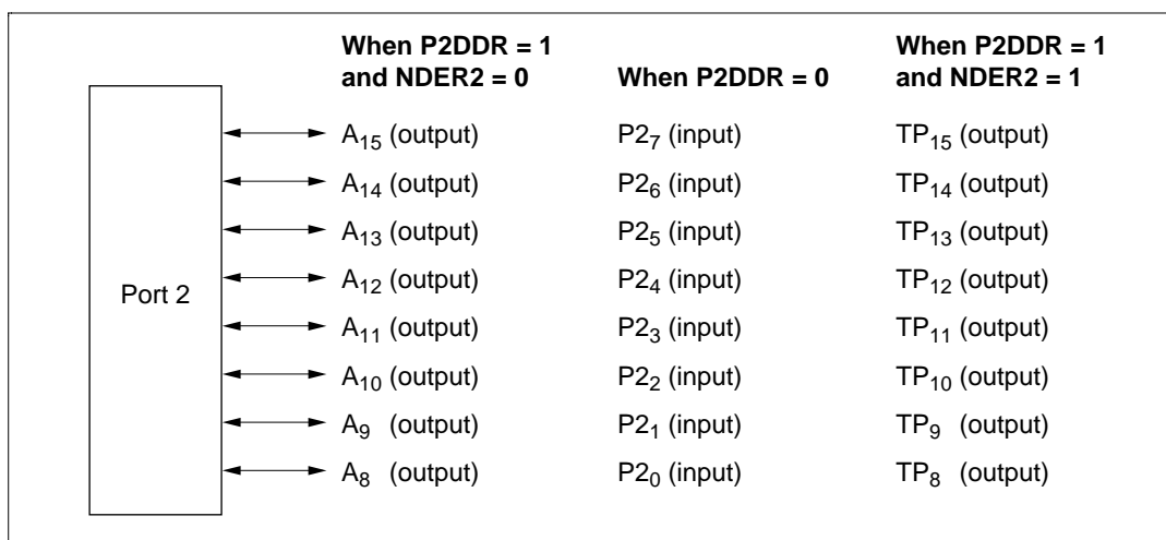
Figure 8.7 Pin Functions in Mode 2 (Port 2)
