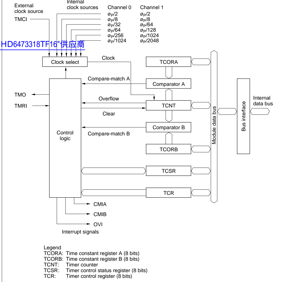
Figure 11.1 Block Diagram of 8-Bit Timer (1 Channel)
