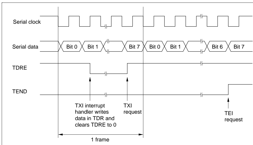
Figure 14.14 Example of SCI Transmit Operation
