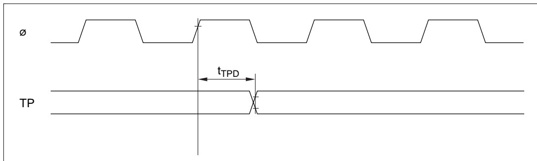
Figure 19.18 Timing Pattern Controller Timing
