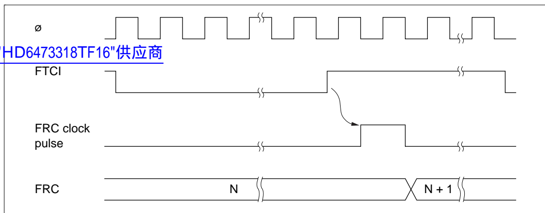
Figure 10.4 Increment Timing for External Clock Source
