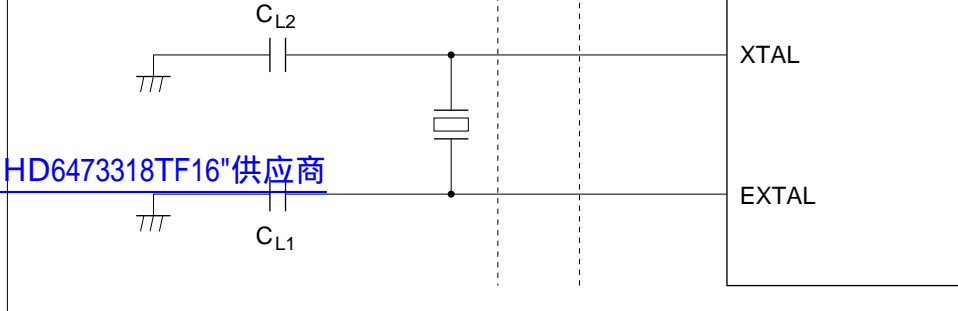
Figure 7.4 Notes on Board Design around External Crystal
