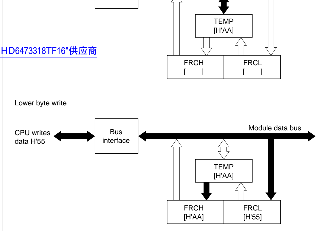
Figure 9.3a Write Access to FRC (when CPU Writes H'AA55)
