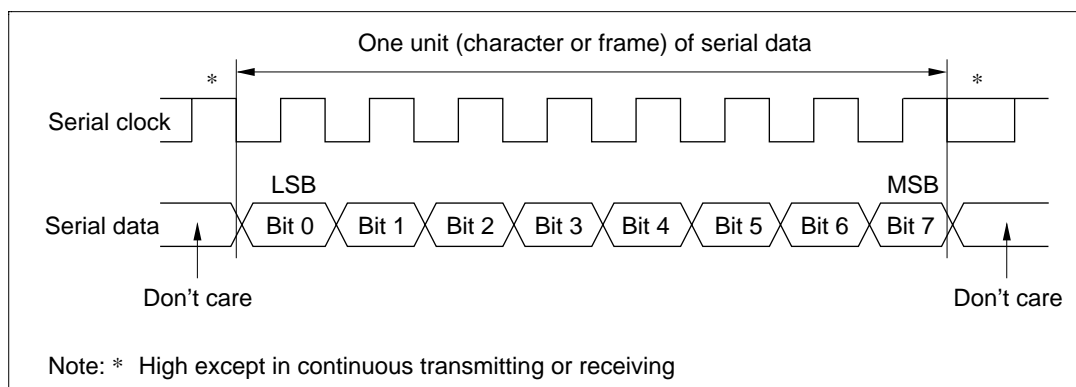
Figure 14.12 Data Format in Synchronous Communication
