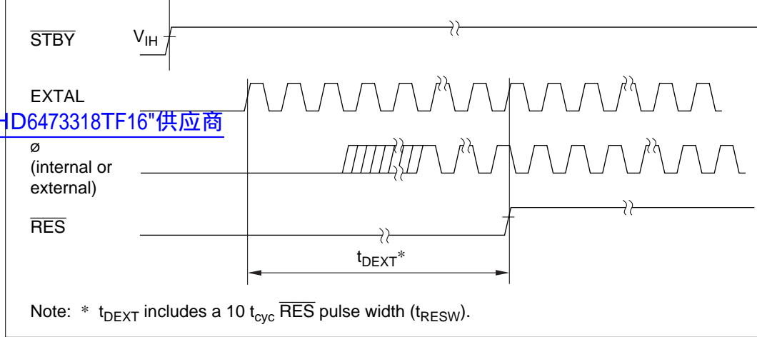
Figure 19.25 External Clock Output Stabilization Delay Time
