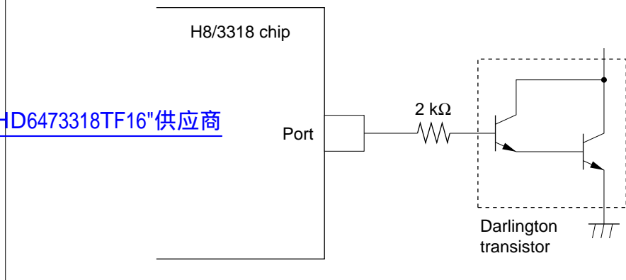
Figure 19.1 Example of Circuit for Driving a Darlington Transistor
