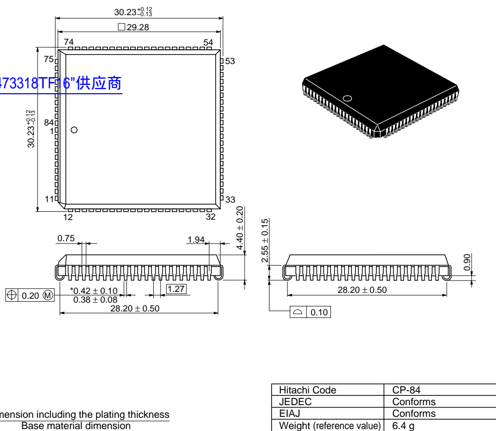
Figure G.3 Package Dimensions (CP-84)
