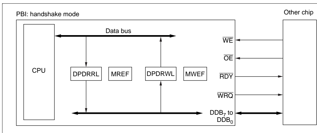
Figure 5.23 Transfers in Handshake Mode
