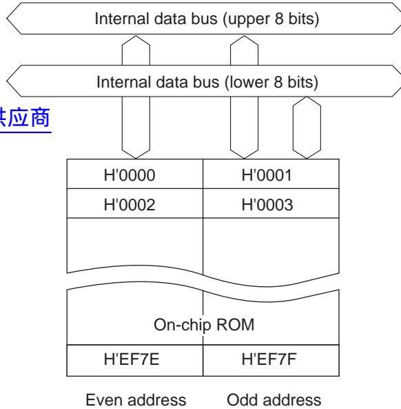
Figure 17.1 Block Diagram of On-Chip ROM (H8/3318 Single-Chip Mode)
