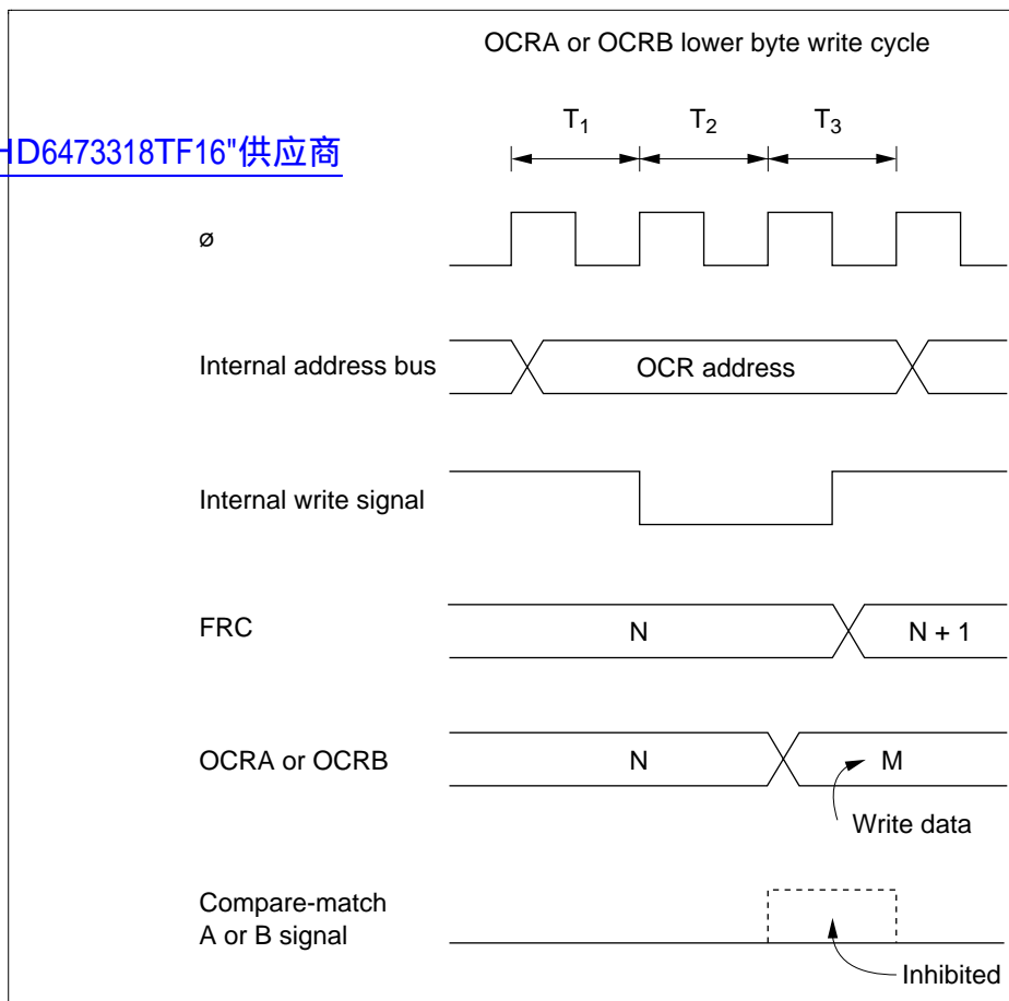
Figure 10.14 Contention between OCR Write and Compare-Match
