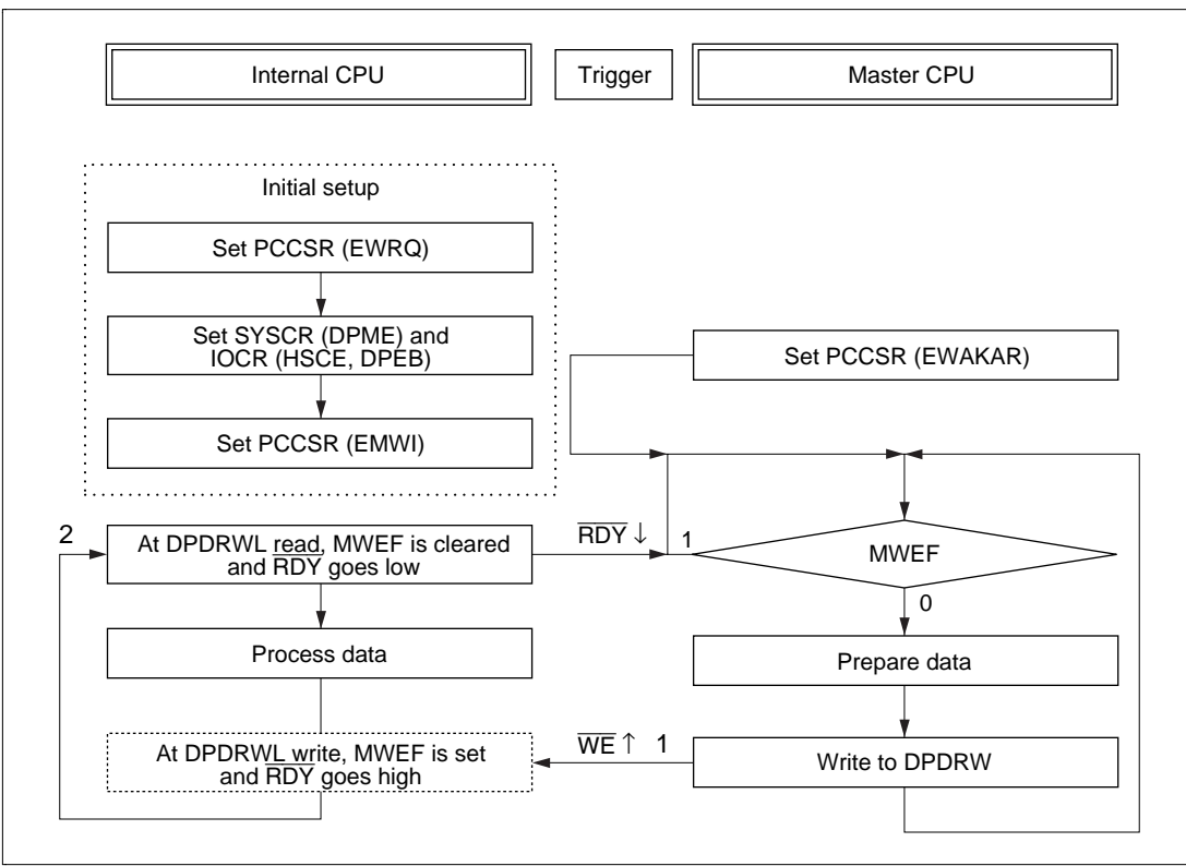
Figure 5.22 Flowchart of Write Operations in DPRAM Direct Word Mode
