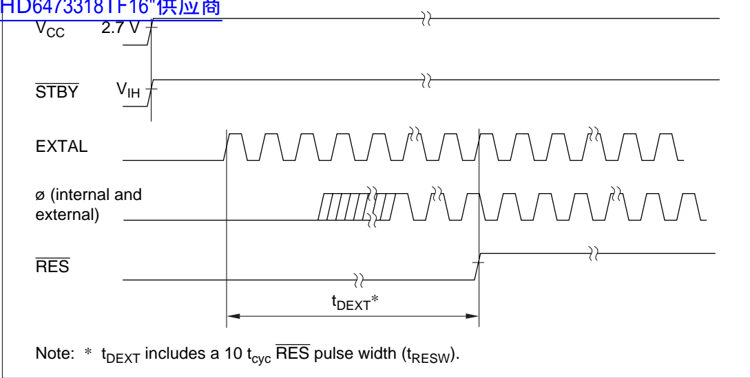
Figure 7.7 External Clock Output Stabilization Delay Time
