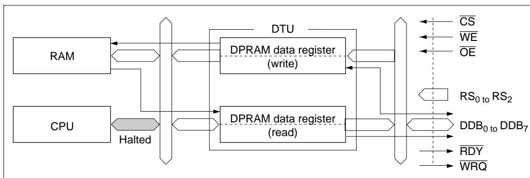
Figure 5.3 Concept of Bound Buffer Mode
