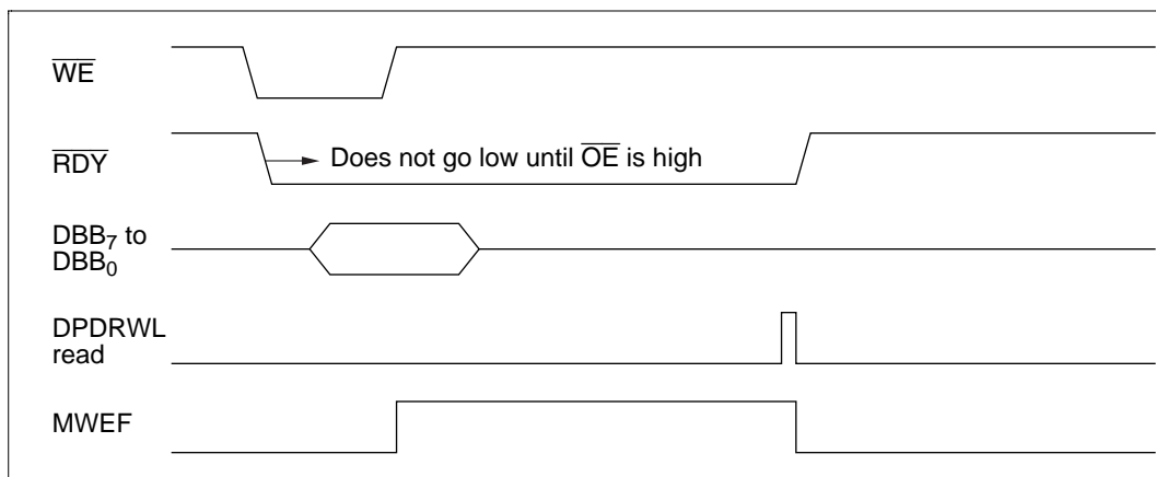
Figure 5.30 Receive Timing in Handshake Mode
