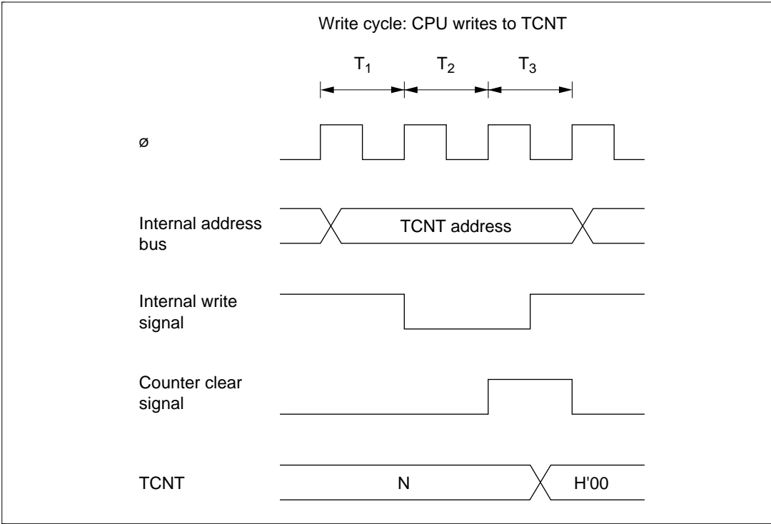
Figure 11.10 TCNT Write-Clear Contention
