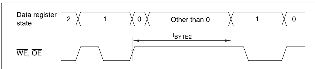
Figure 19.22 (b) Access Interval in Bound Buffer Mode (without \overline{WRQ} )
