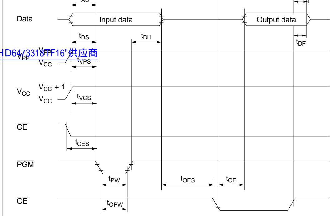
Figure 17.5 PROM Program/Verify Timing
