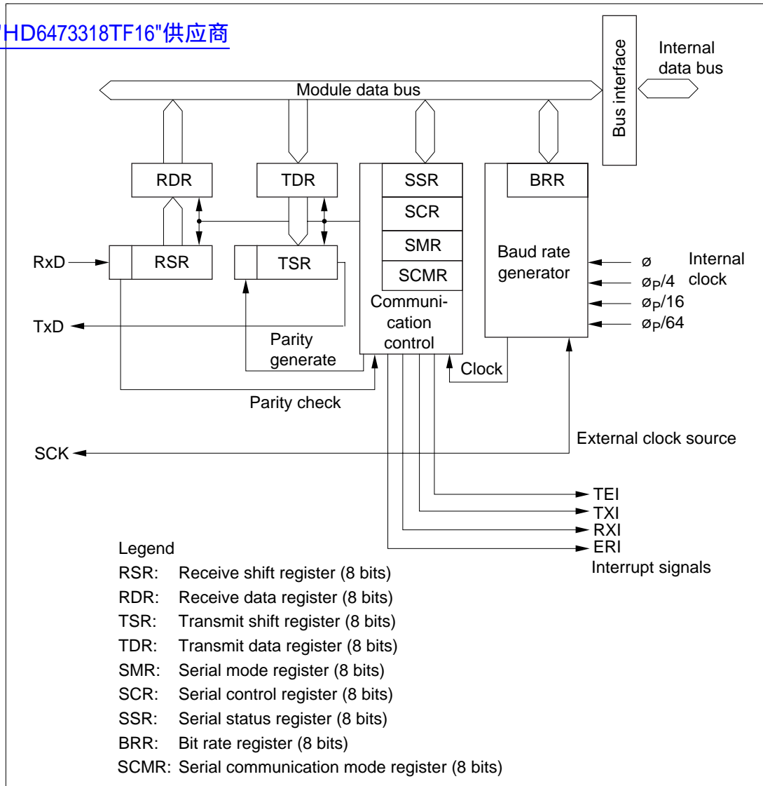
Figure 14.1 Block Diagram of Serial Communication Interface
