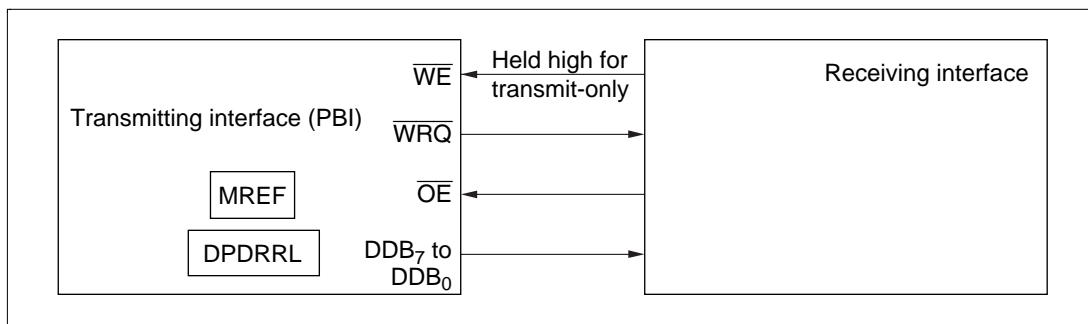
Figure 5.27 Transmitting in Handshake Mode
