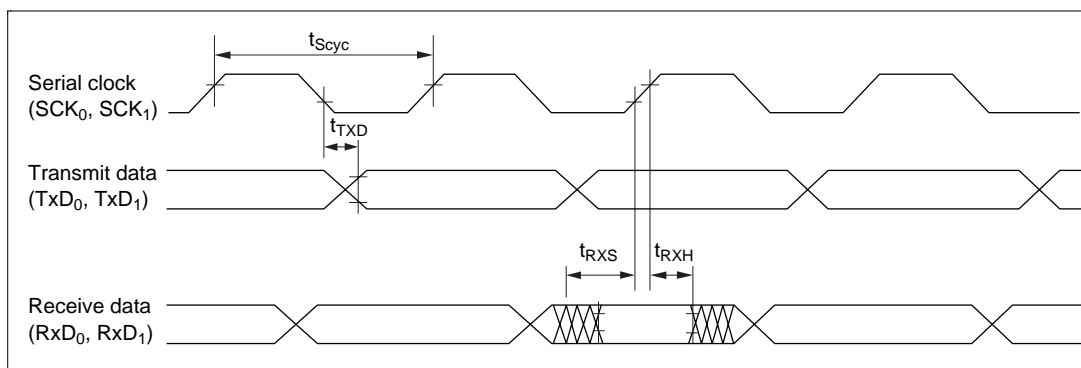
Figure 19.15 SCI Input/Output Timing (Synchronous Mode)
