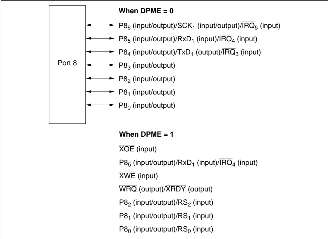
Figure 8.19 Pin Functions in Modes 1 and 2 (Port 8)
