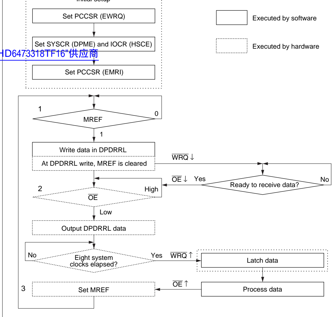
Figure 5.25 Flowchart of Transmit Operations in Handshake Mode
