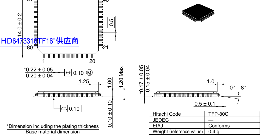
Figure G.2 Package Dimensions (TFP-80C)
