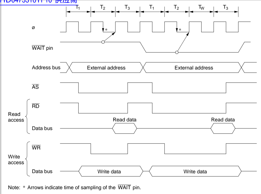
Figure 6.4 Pin Auto-Wait Mode
