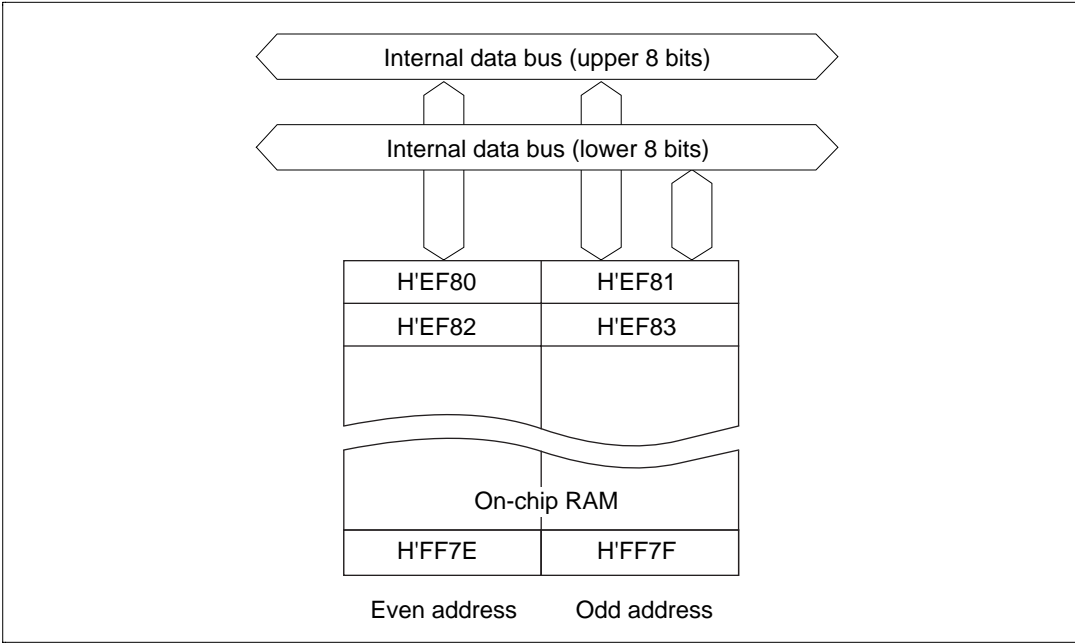
Figure 16.1 Block Diagram of On-Chip RAM
