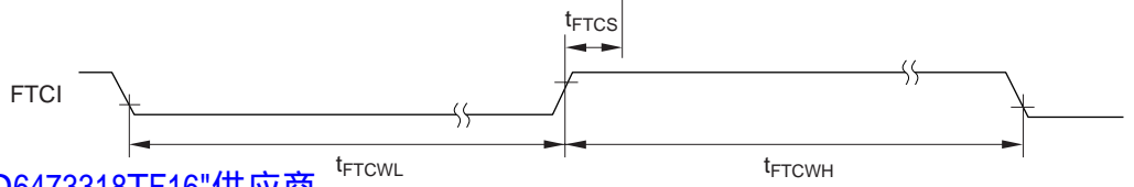
Figure 19.11 External Clock Input Timing for Free-Running Timer
