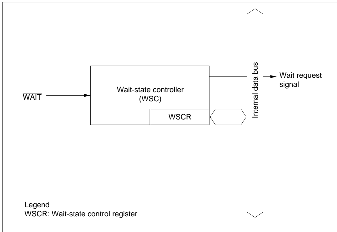
Figure 6.1 Block Diagram of Wait-State Controller
