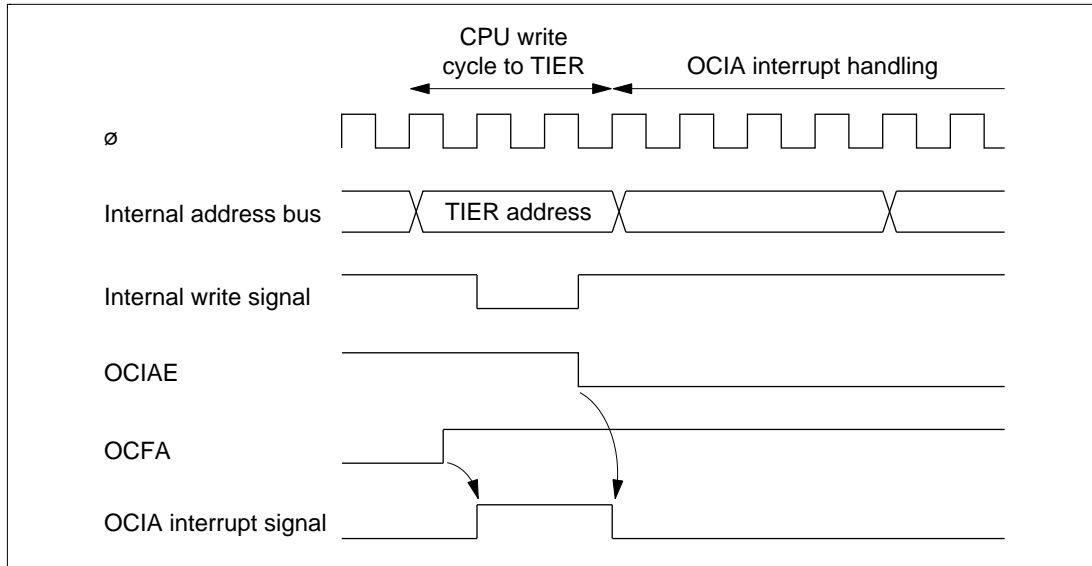
Figure 4.7 Contention between Interrupt and Disabling Instruction
