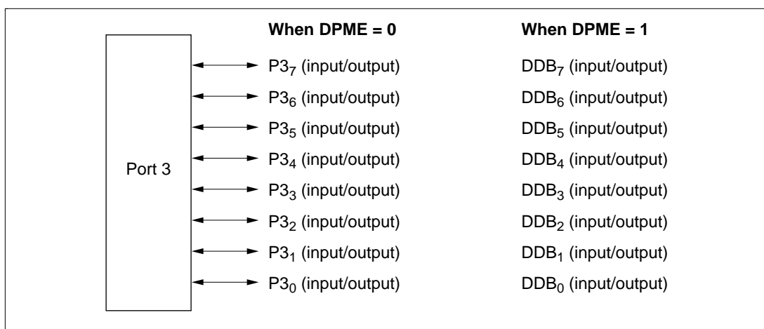
Figure 8.11 Pin Functions in Mode 3 (Port 3)
