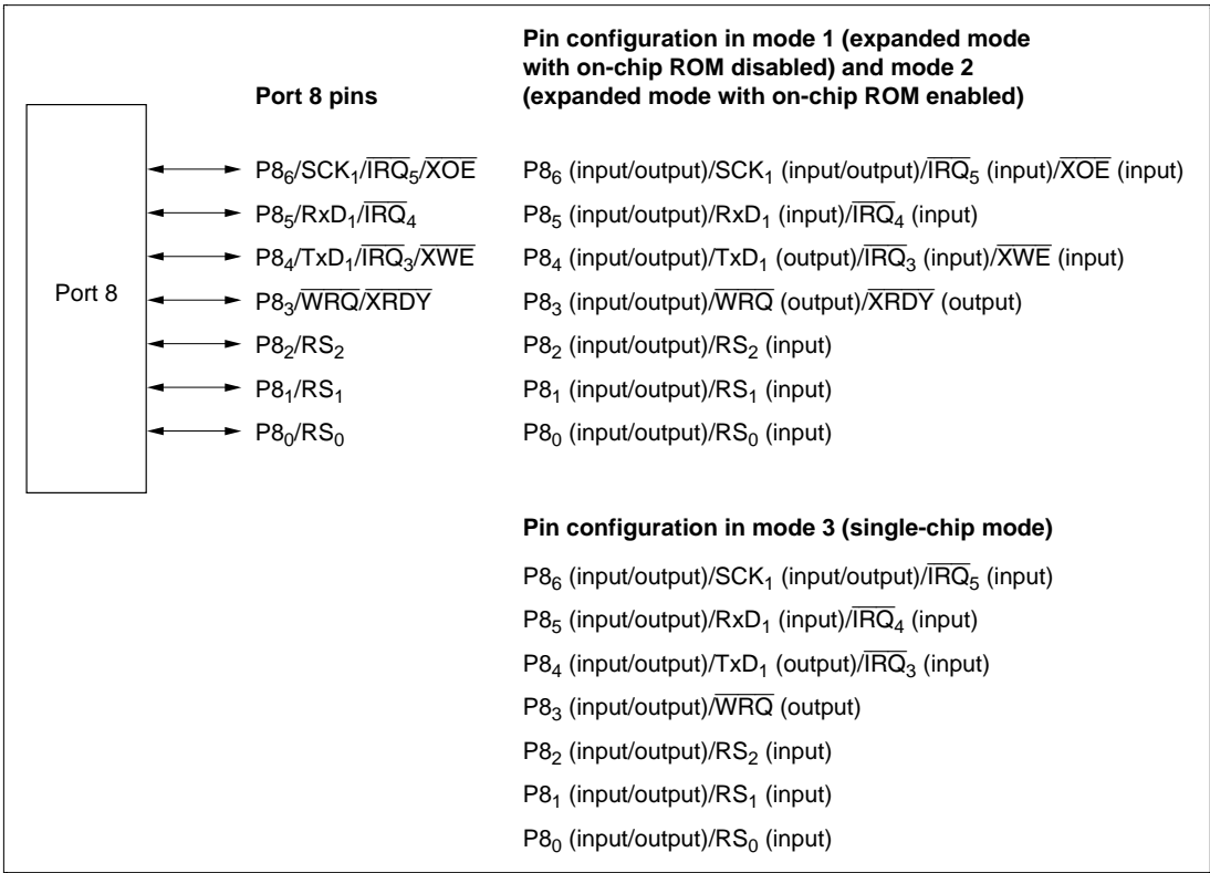
Figure 8.18 Port 8 Pin Configuration
