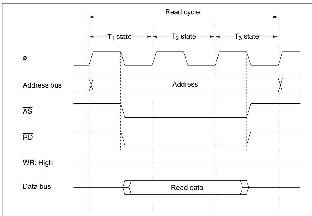
Figure 2.17 (a) External Device Access Timing (Read)
