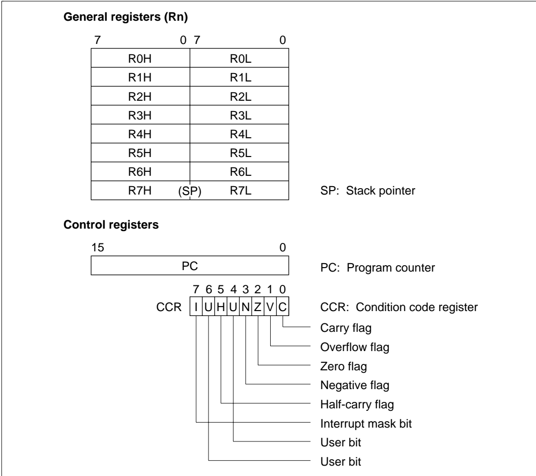
Figure 2.1 CPU Registers
