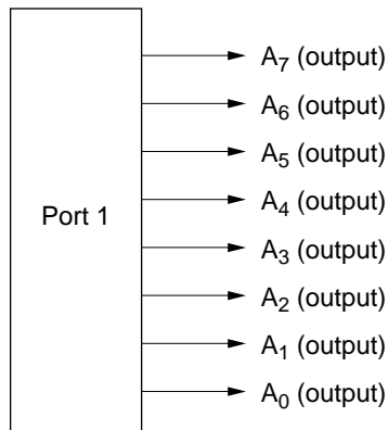
Figure 8.2 Pin Functions in Mode 1 (Port 1)
