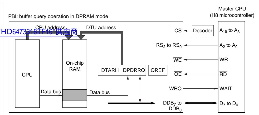
Figure 5.14 Buffer Query in DPRAM Mode
