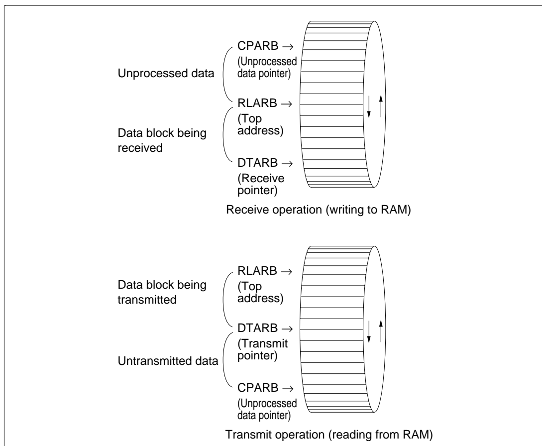
Figure 5.11 Pointer Operation in Ring Buffer
