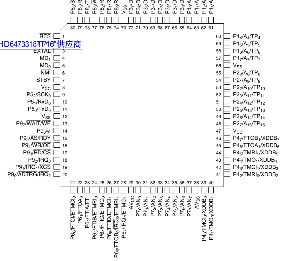
Figure 1.3 Pin Arrangement (FP-80A and TFP-80C, Top View)
