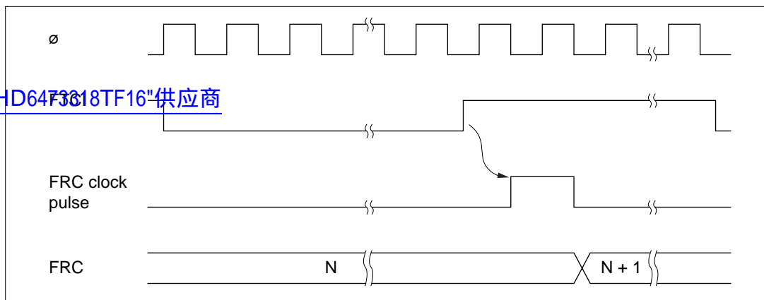
Figure 9.5 Increment Timing for External Clock Source
