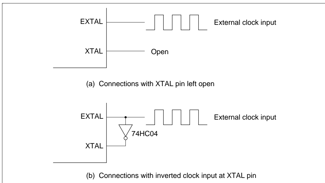
Figure 7.5 External Clock Input (Example)
