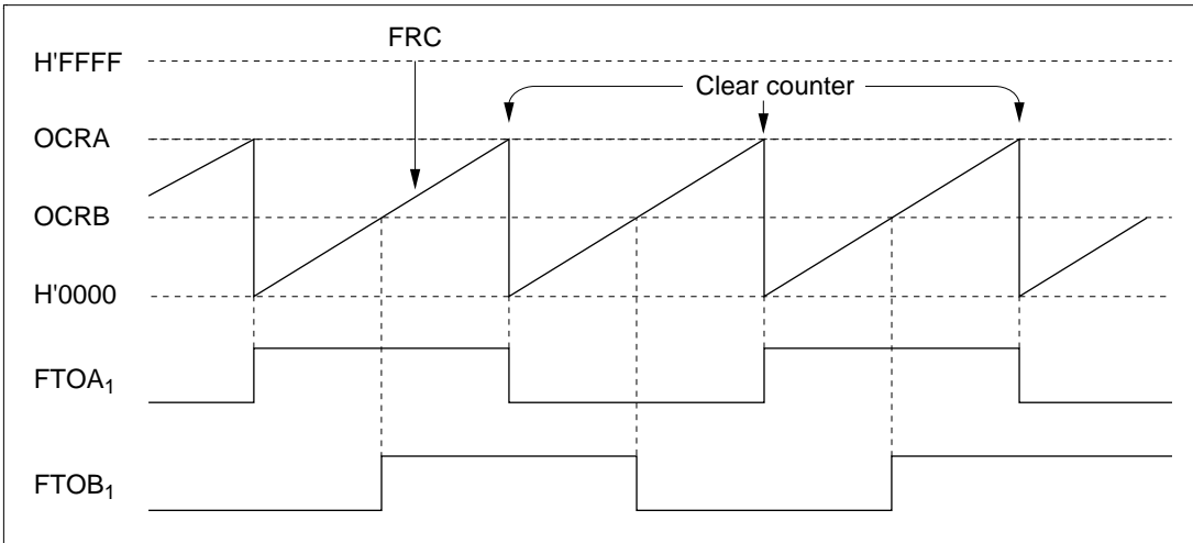
Figure 10.11 Square-Wave Output (Example)
