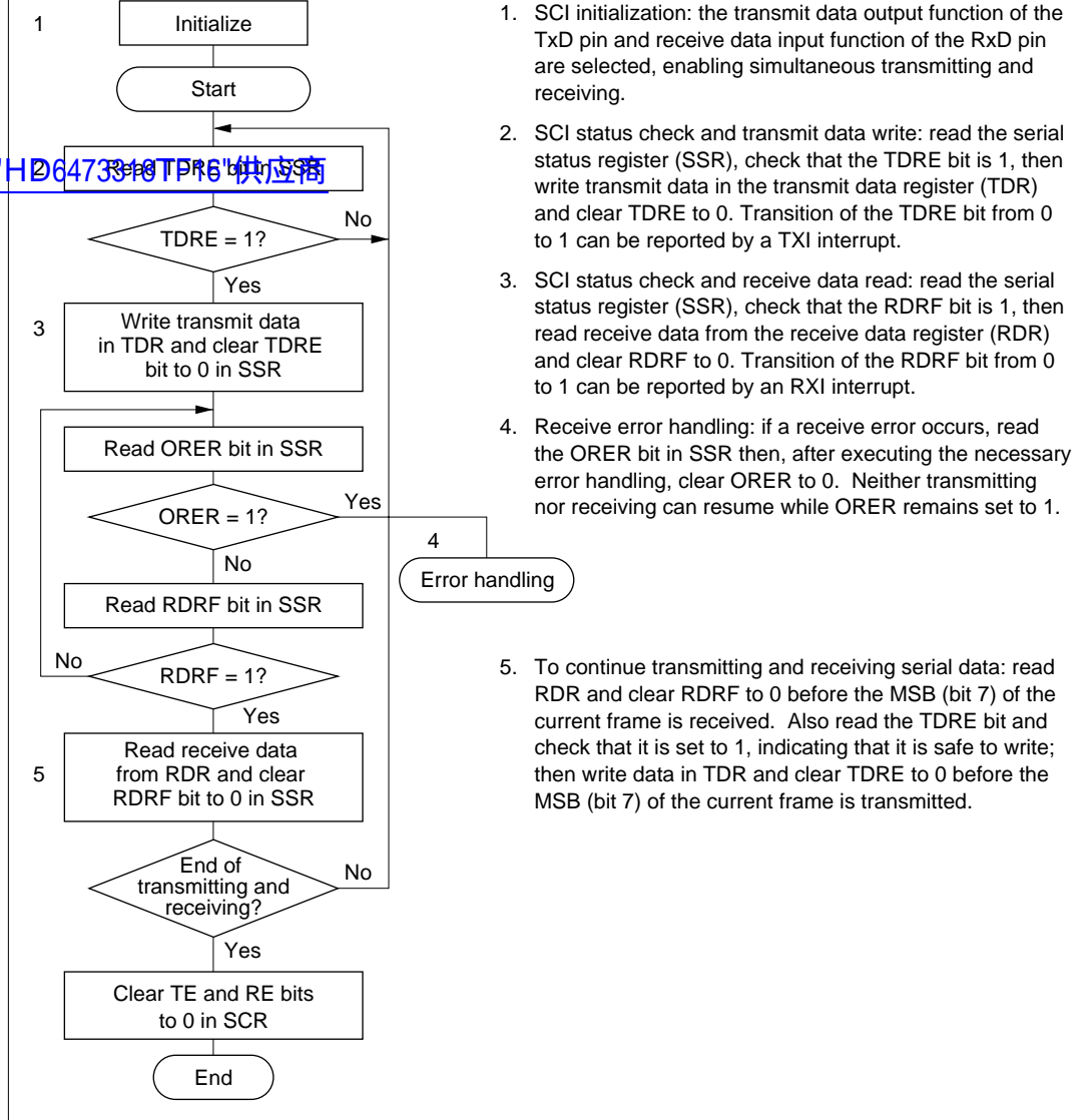
Figure 14.17 Sample Flowchart for Serial Transmitting and Receiving
