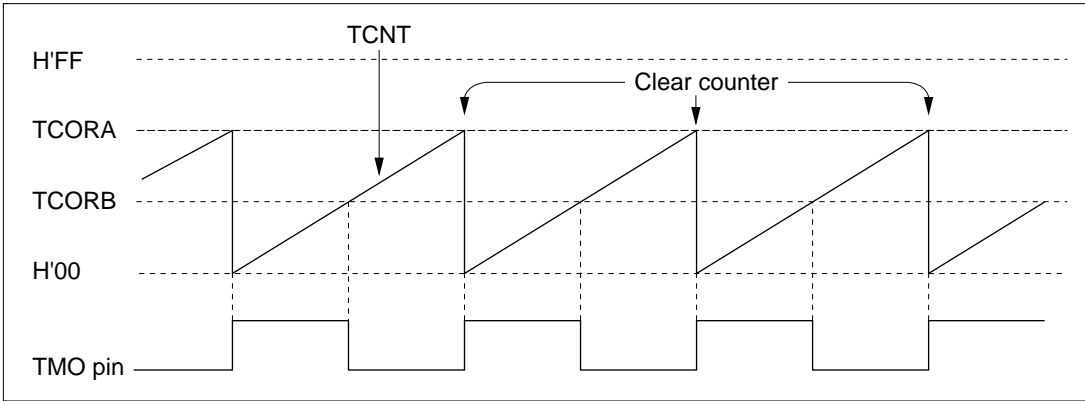
Figure 11.9 Example of Pulse Output
