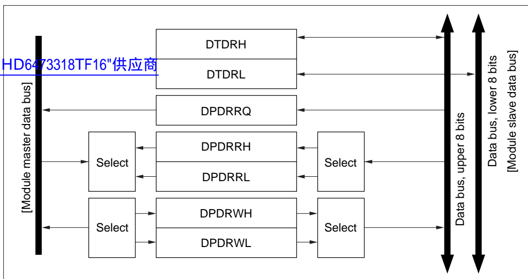
Figure 5.9 Concept of Data Bus Circuits
