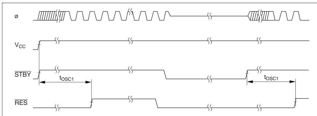
Figure 19.8 Clock Settling Timing
