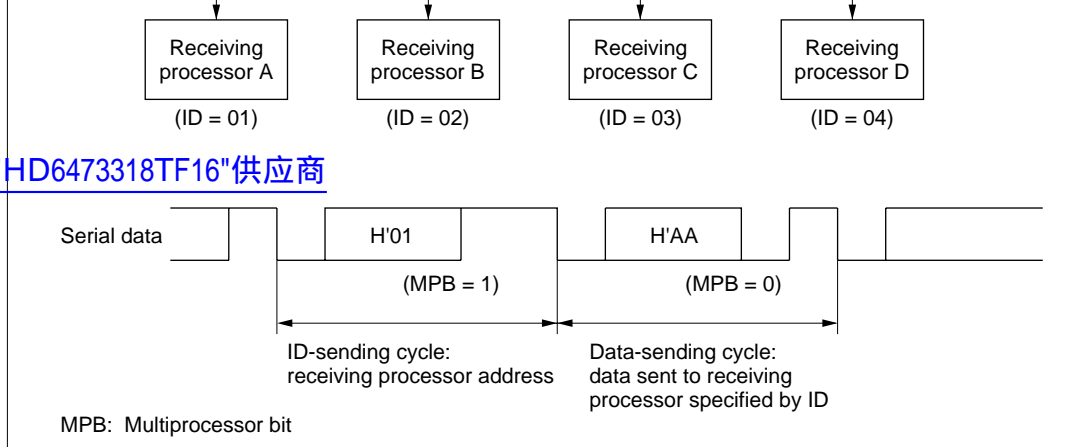
Figure 14.9 Example of Communication among Processors using Multiprocessor Format (Sending Data H'AA to Receiving Processor A)
