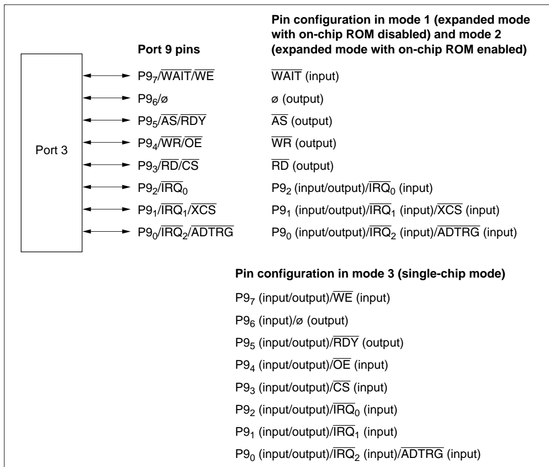
Figure 8.21 Port 9 Pin Configuration
