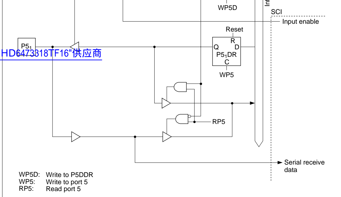
Figure C.5 (b) Port 5 Block Diagram (Pin P5 1 )
