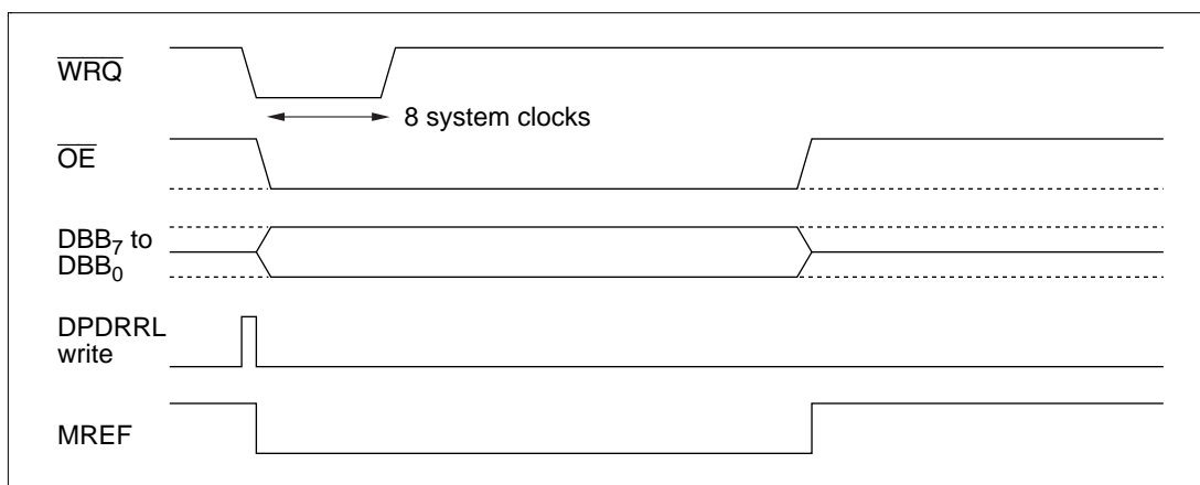
Figure 5.28 Transmit Timing in Handshake Mode
