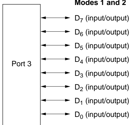
Figure 8.10 Pin Functions in Modes 1 and 2 (Port 3)
