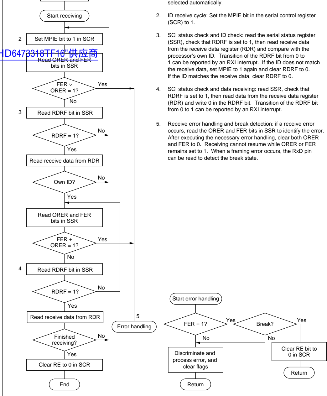
Figure 14.10 Sample Flowchart for Receiving Multiprocessor Serial Data
