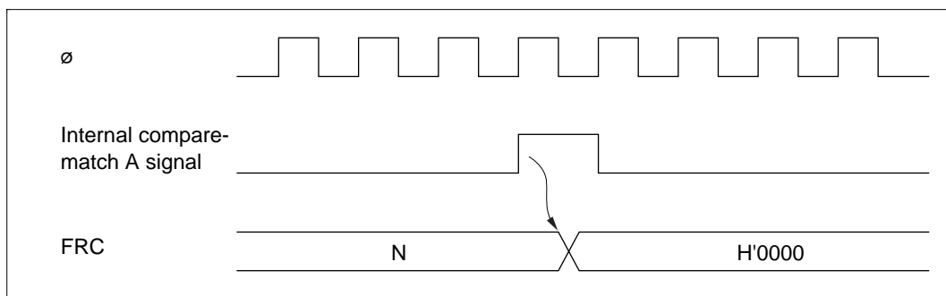
Figure 10.6 Clearing of FRC by Compare-Match A
