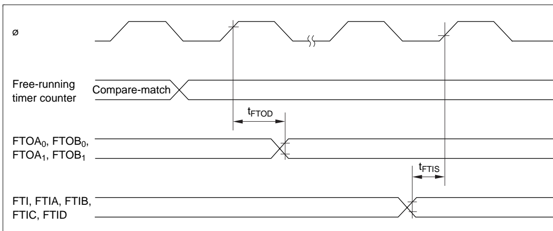
Figure 19.10 Free-Running Timer Input/Output Timing
