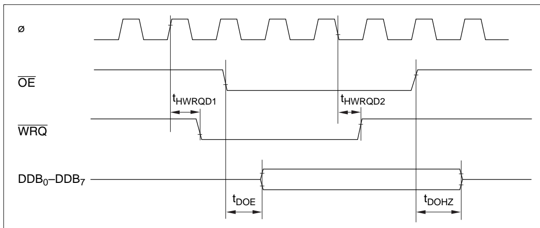
Figure 19.24 Transmit Timing in Handshake Mode
