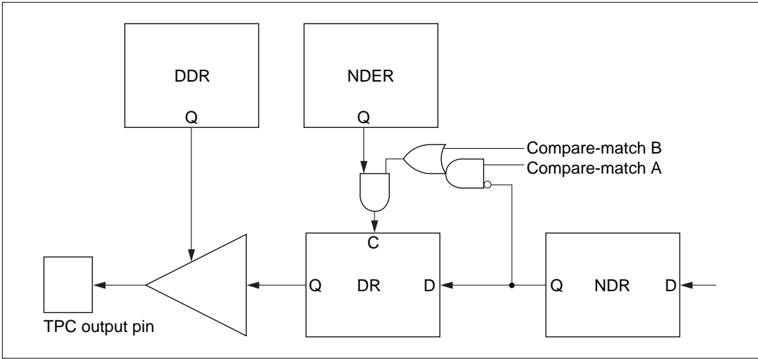
Figure 12.8 Non-Overlapping TPC Output
