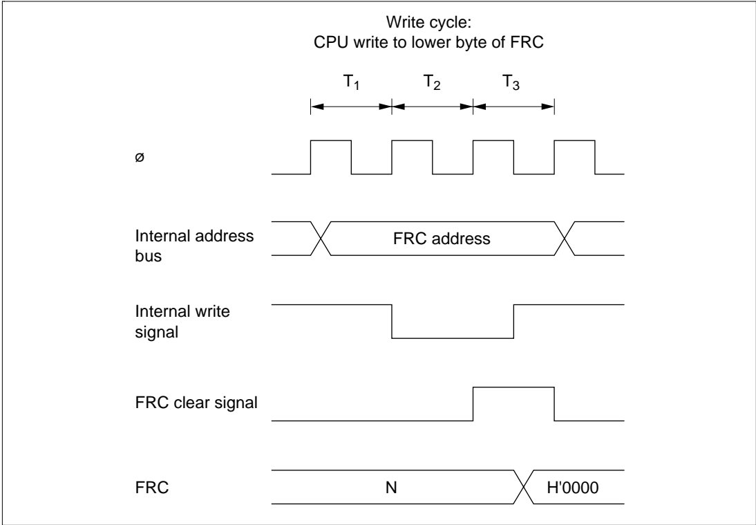
Figure 9.16 FRC Write-Clear Contention
