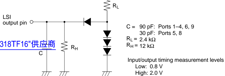
Figure 19.3 Output Load Circuit
