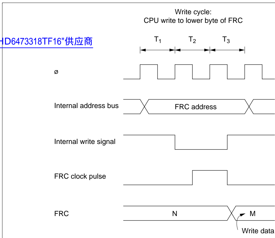
Figure 9.17 FRC Write-Increment Contention
