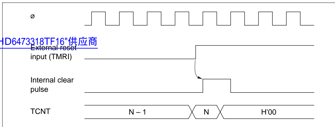
Figure 11.7 Timing of External Reset
