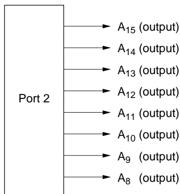
Figure 8.6 Pin Functions in Mode 1 (Port 2)
