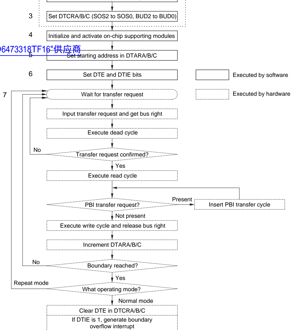
Figure 5.13 I/O Transfer Flowchart
