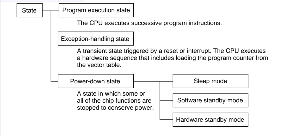
Figure 2.11 Operating States
