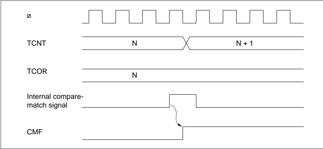
Figure 11.4 Setting of Compare-Match Flags
