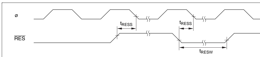
Figure 19.6 Reset Input Timing
