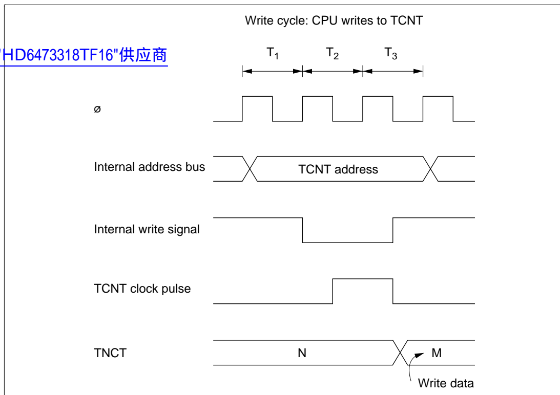
Figure 11.11 TCNT Write-Increment Contention
