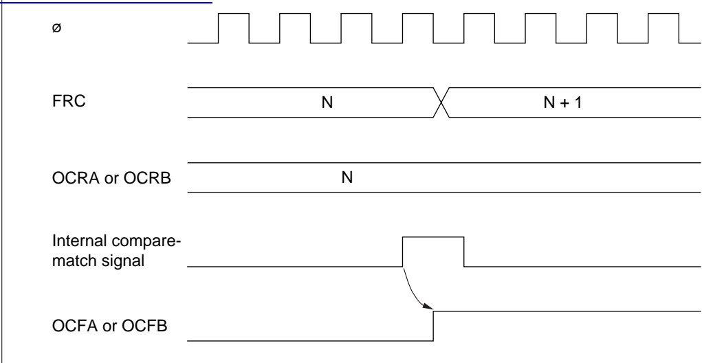
Figure 9.13 Setting of Output Compare Flags
