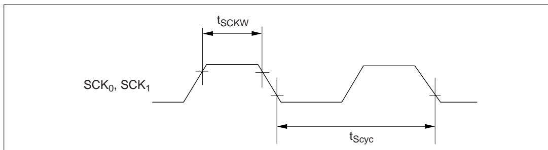
Figure 19.16 SCI Input Clock Timing
