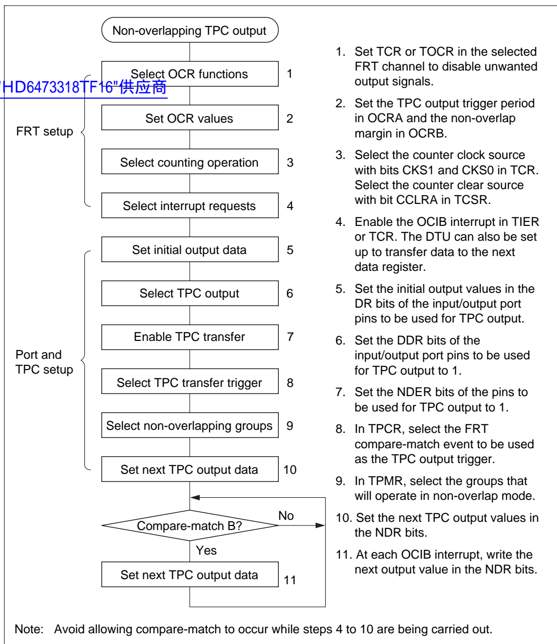
Figure 12.6 Setup Procedure for Non-Overlapping TPC Output (Example)
