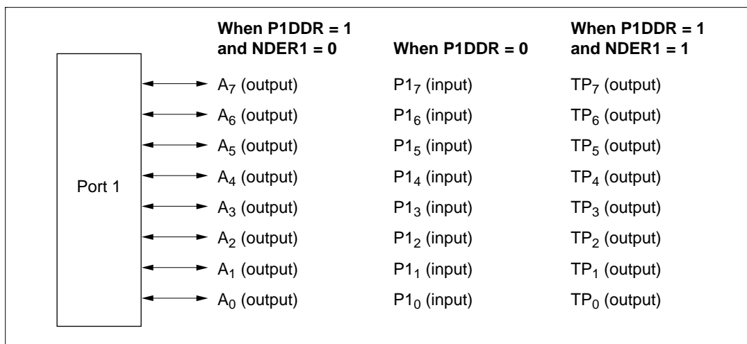
Figure 8.3 Pin Functions in Mode 2 (Port 1)
