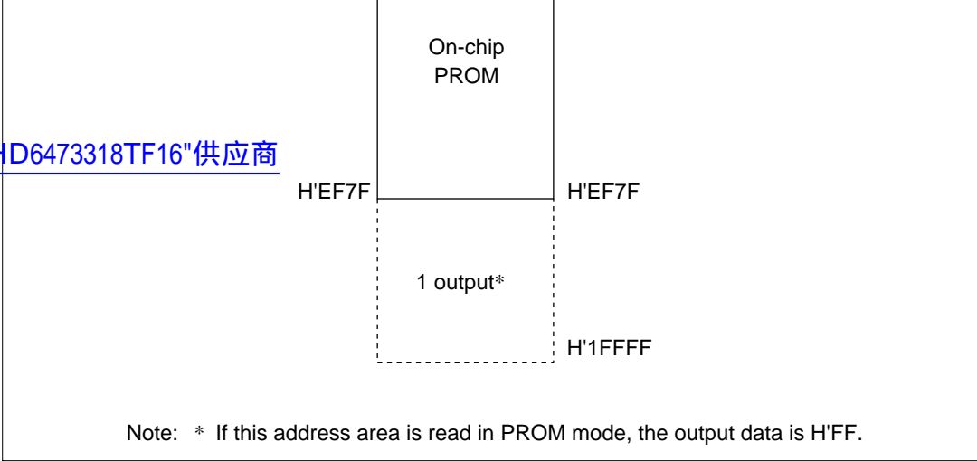
Figure 17.3 H8/3318 Memory Map in PROM Mode
