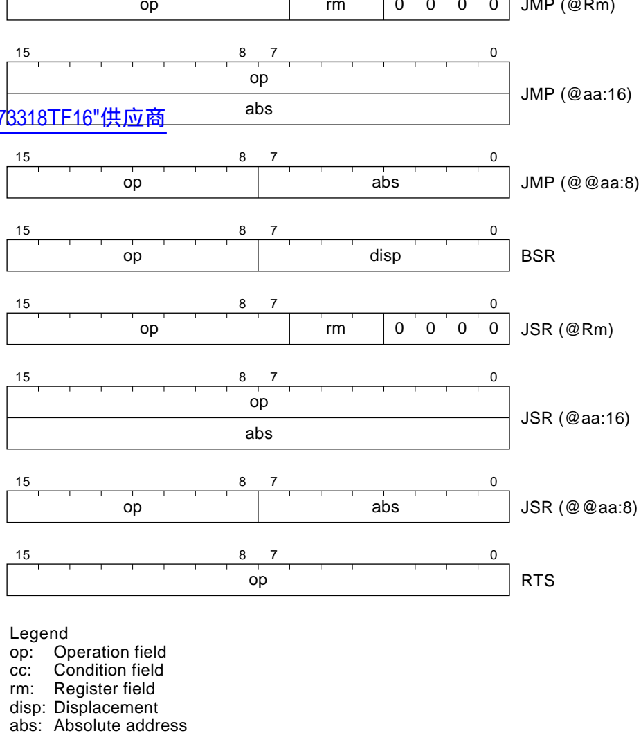
Figure 2.8 Branching Instruction Codes
