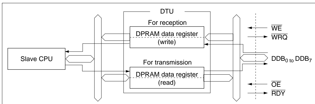
Figure 5.5 Concept of Handshake Mode
