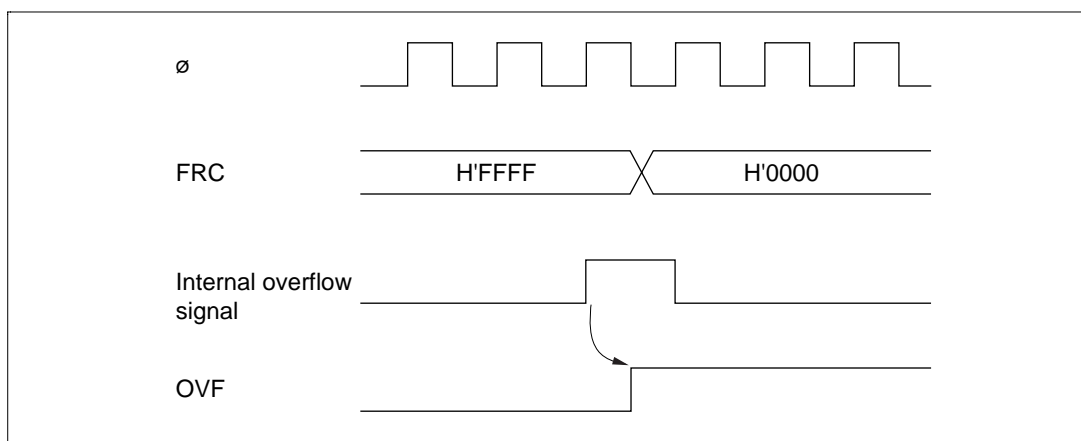
Figure 10.10 Setting of Overflow Flag (OVF)
