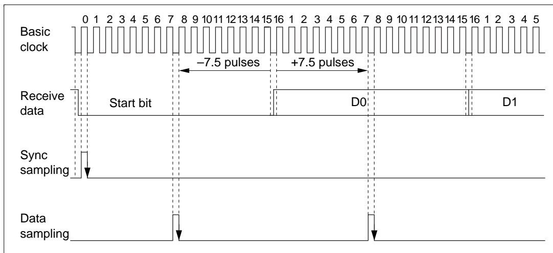
Figure 14.18 Sampling Timing (Asynchronous Mode)
