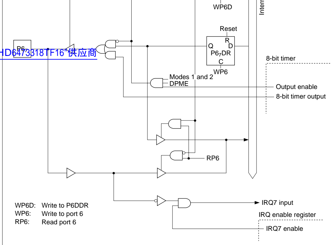
Figure C.6 (f) Port 6 Block Diagram (Pin P6 7 )
