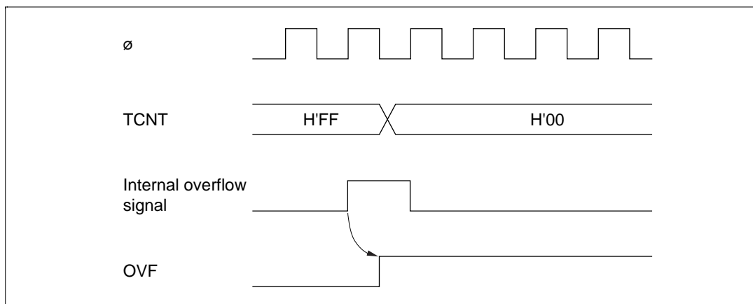
Figure 11.8 Setting of Overflow Flag (OVF)
