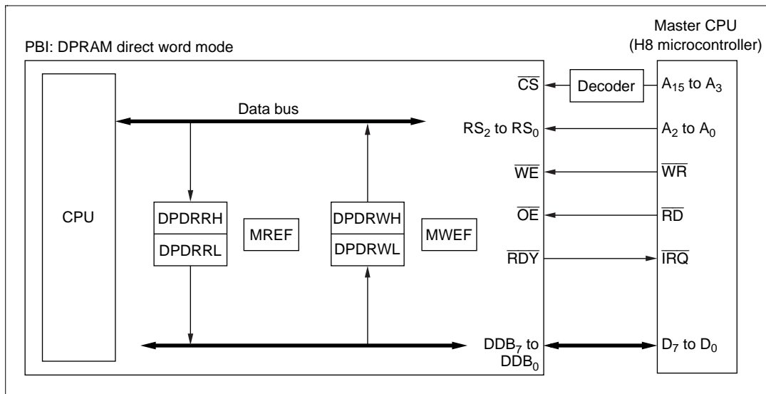
Figure 5.20 Read/Write Access in DPRAM Direct Word Mode
