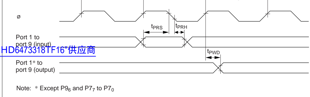
Figure 19.17 I/O Port Input/Output Timing
