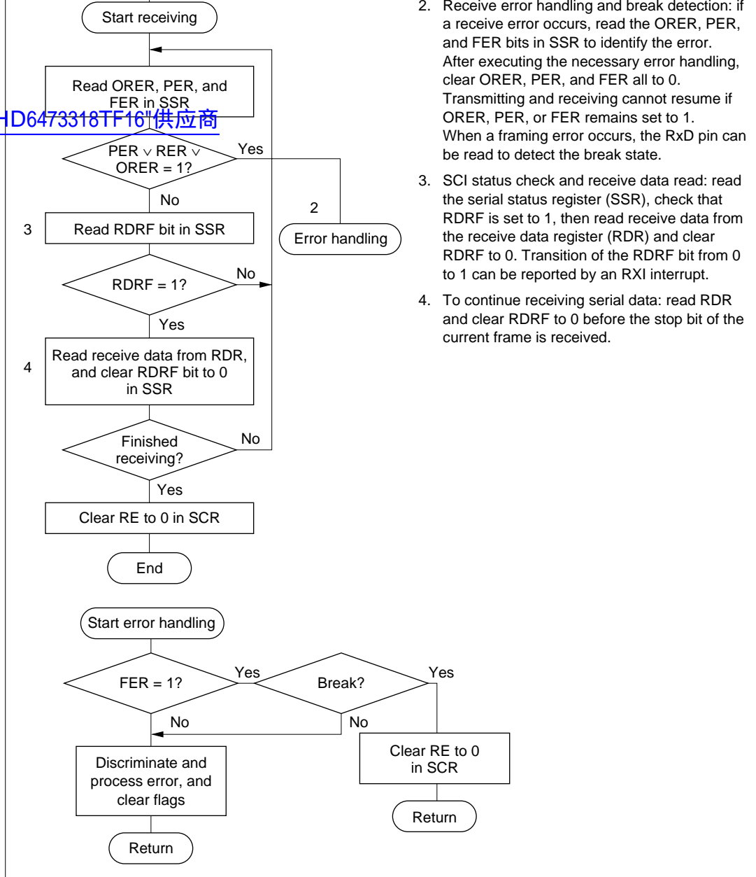
Figure 14.7 Sample Flowchart for Receiving Serial Data
