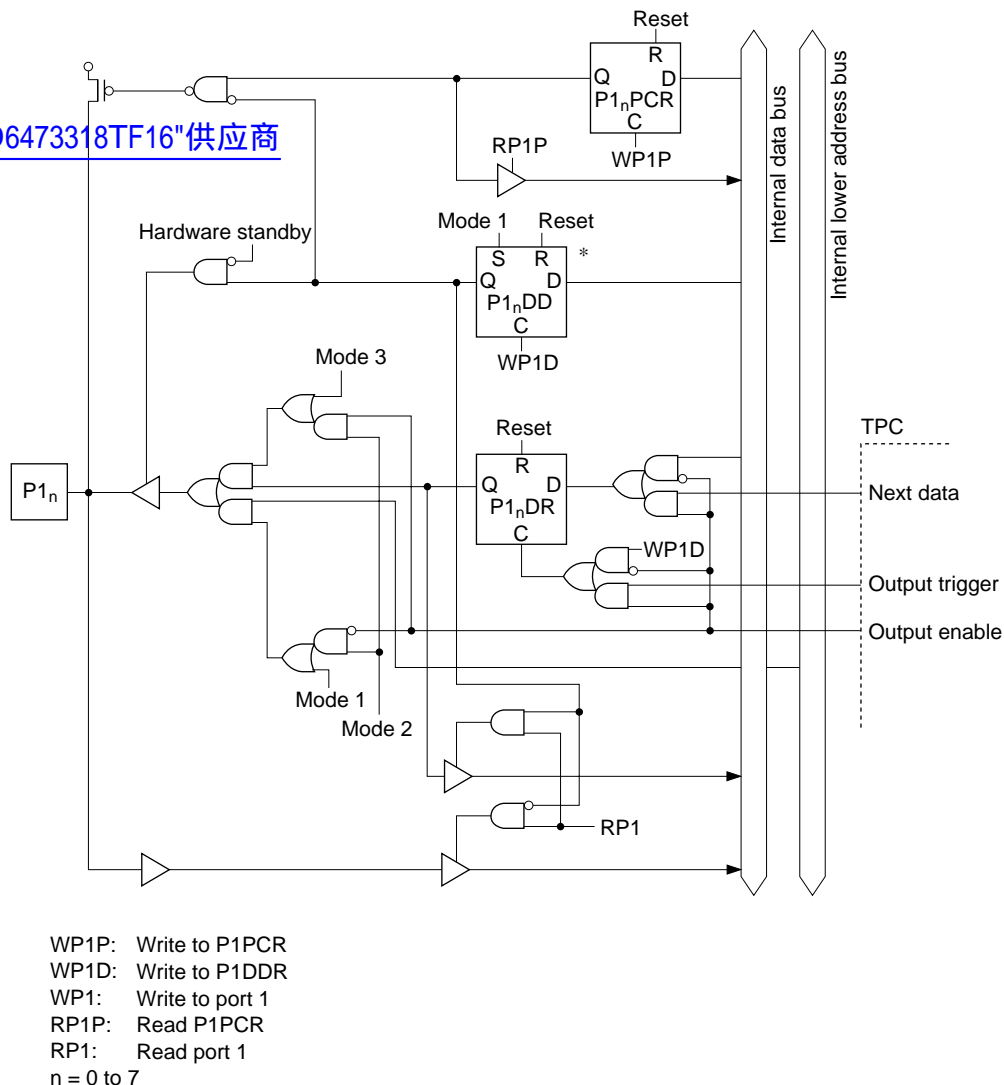
Figure C.1 Port 1 Block Diagram
