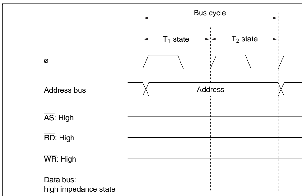
Figure 2.14 Pin States during On-Chip Memory Access Cycle
