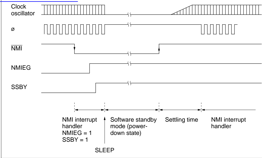
Figure 18.1 NMI Timing in Software Standby Mode
