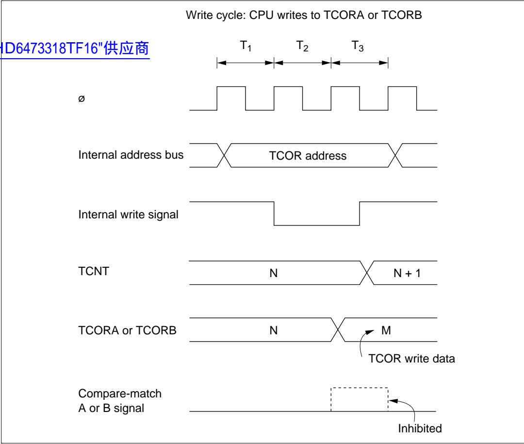
Figure 11.12 Contention between TCOR Write and Compare-Match
