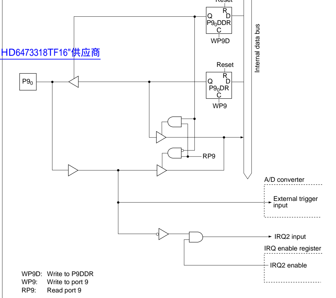
Figure C.9 (a) Port 9 Block Diagram (Pin P9 0 )
