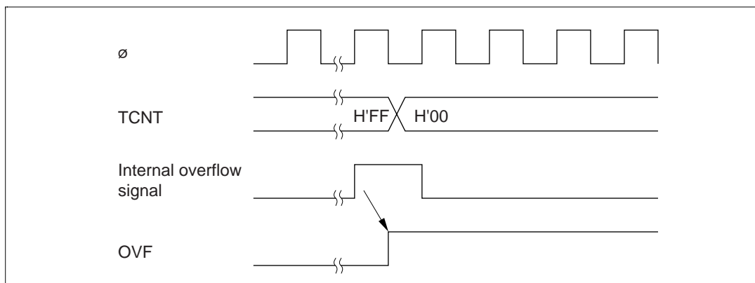
Figure 13.5 Setting the OVF Bit
