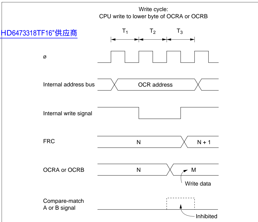
Figure 9.18 Contention between OCR Write and Compare-Match
