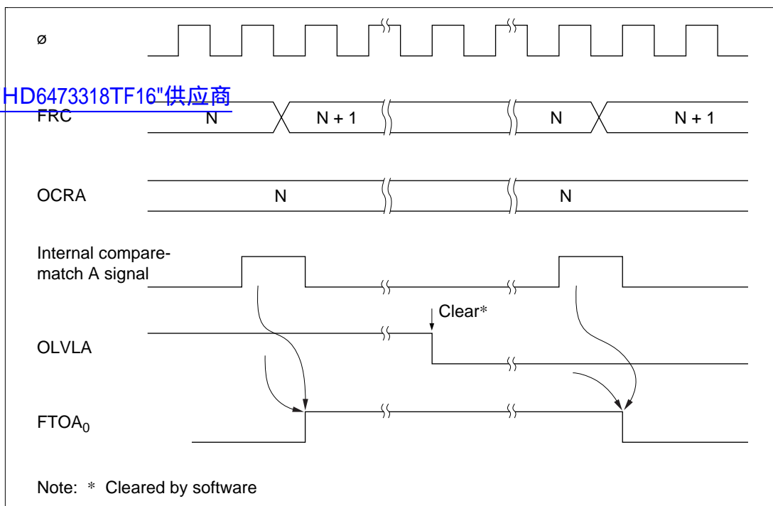
Figure 9.6 Timing of Output Compare A
