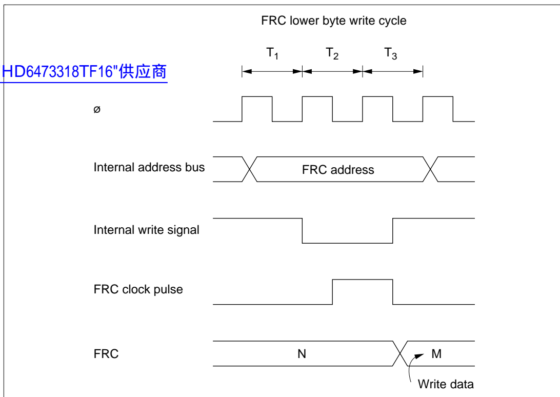
Figure 10.13 FRC Write-Increment Contention
