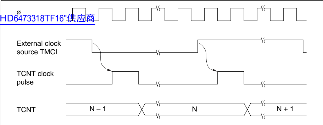
Figure 11.3 Count Timing for External Clock Input
