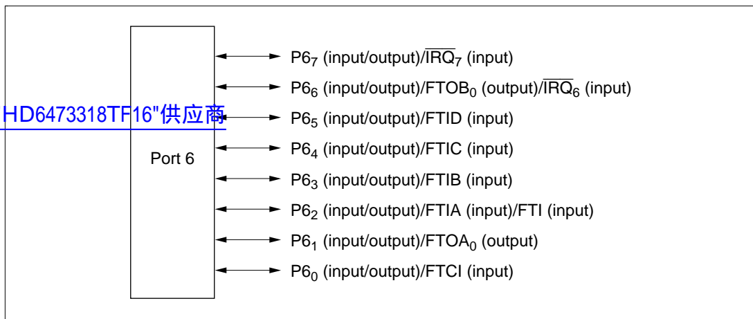
Figure 8.16 Pin Functions in Mode 3 (Port 6)
