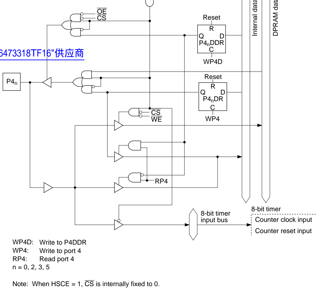
Figure C.4 (a) Port 4 Block Diagram (Pins P4 0 , P4 2 , P4 3 , P4 5 )
