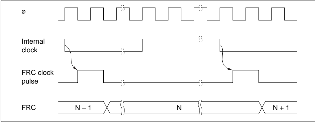
Figure 9.4 Increment Timing for Internal Clock Source
