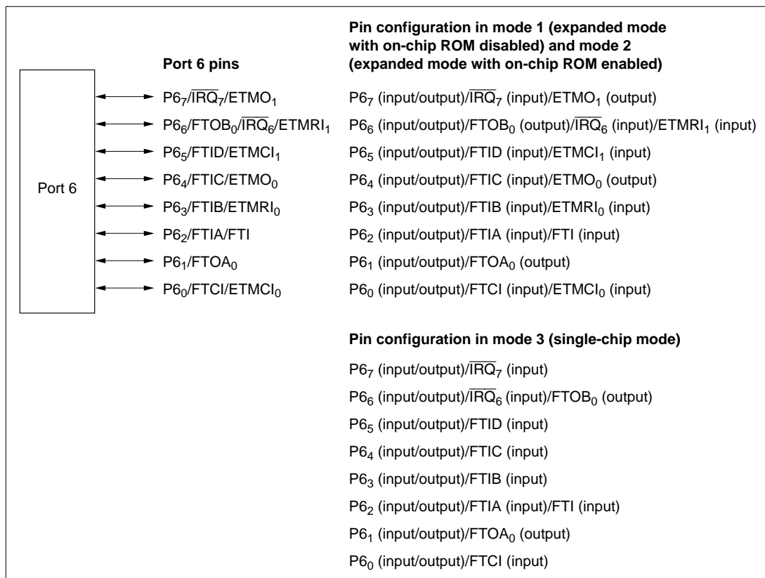
Figure 8.14 Port 6 Pin Configuration
