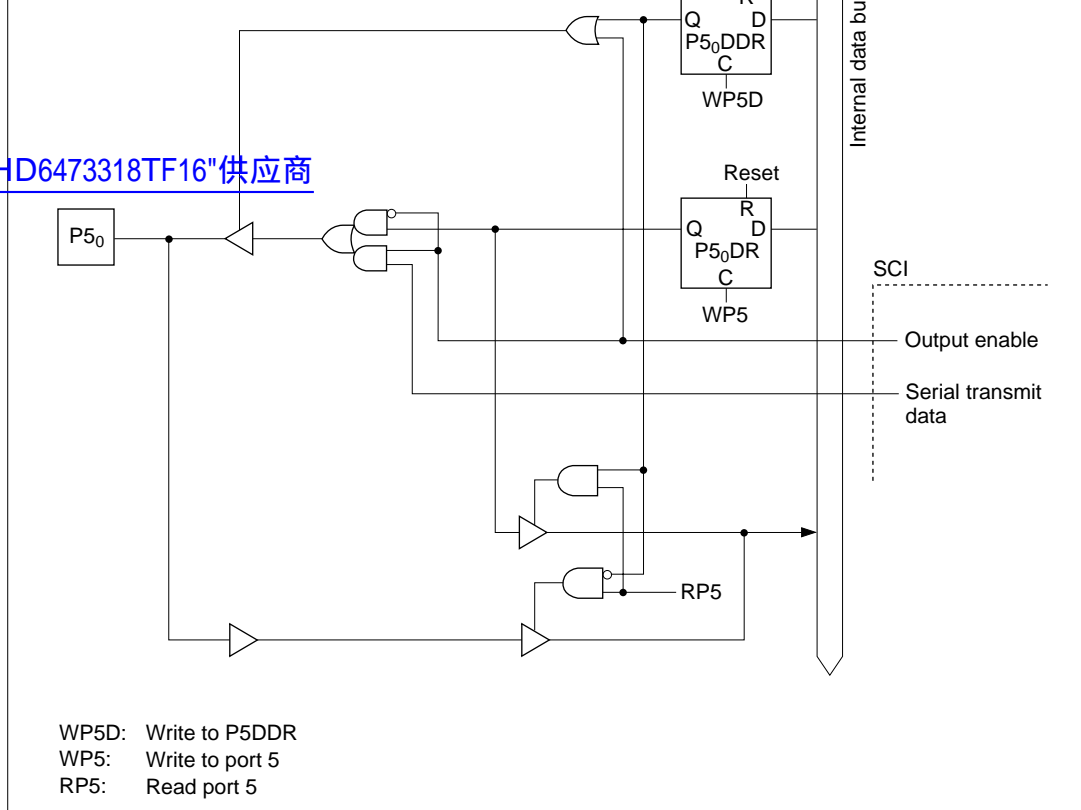
Figure C.5 (a) Port 5 Block Diagram (Pin P5 0 )
