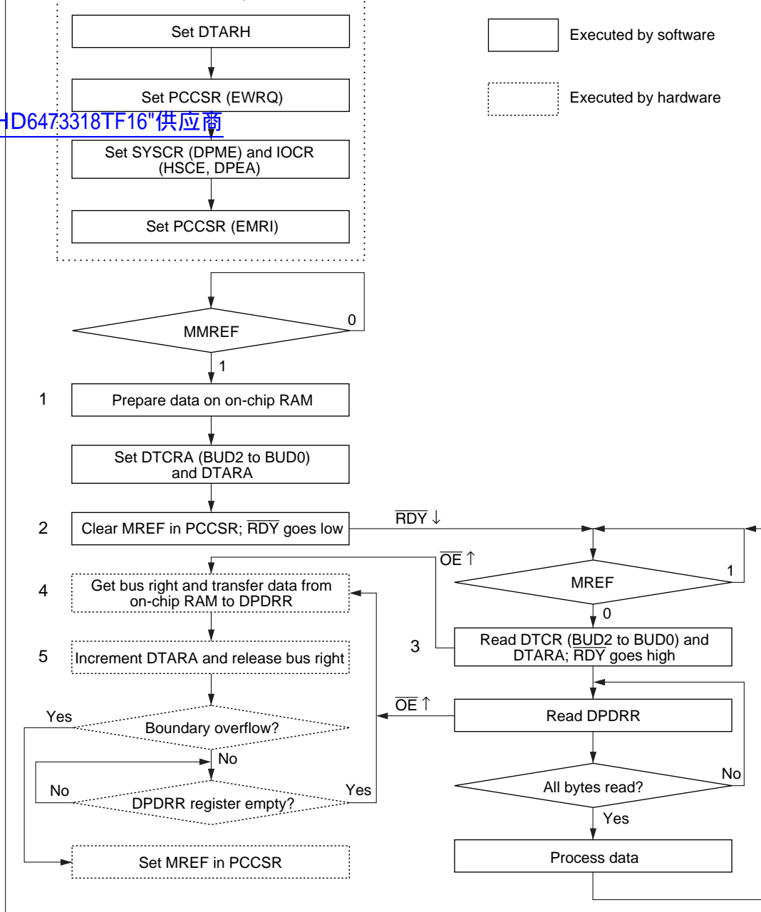
Figure 5.17 Flowchart of Read Operations in DPRAM Bound Buffer Mode
