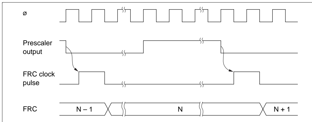
Figure 10.3 Increment Timing for Internal Clock Source
