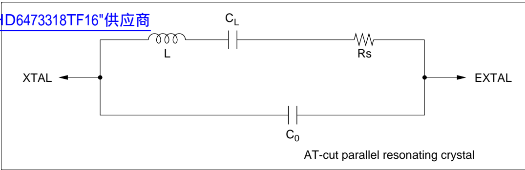
Figure 7.3 Equivalent Circuit of External Crystal
