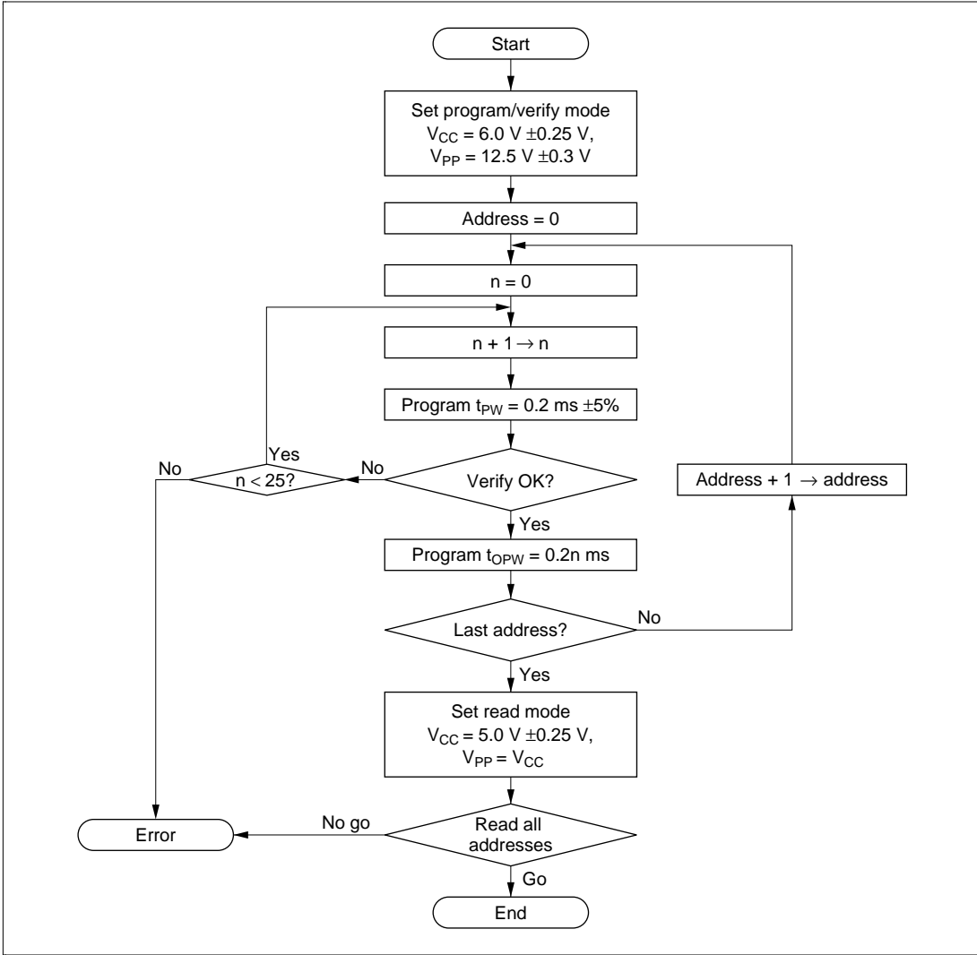
Figure 17.4 High-Speed Programming Flowchart
