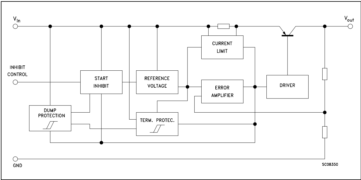
Figure 1. Block diagram
