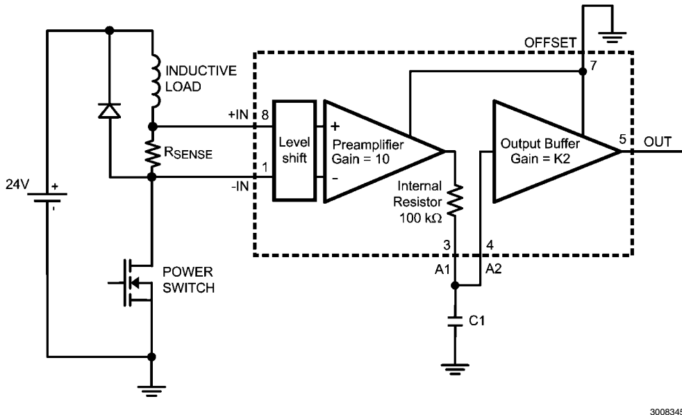
FIGURE 9. Low Side Current Sensing Application with Large Common Mode Transients
