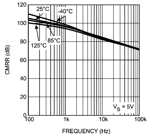
CMRR vs. Frequency at V_S = 5\text{V}
