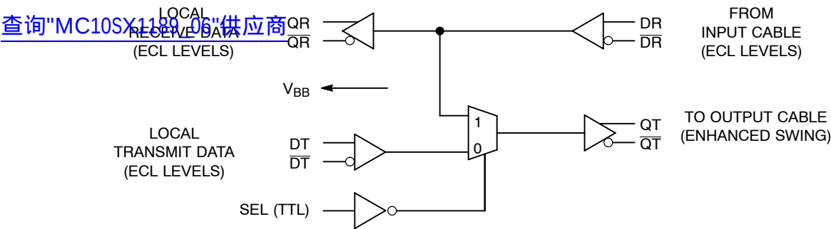
Figure 2. LOGIC DIAGRAM
