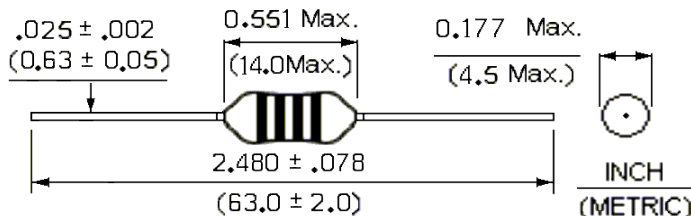
Mechanical drawing
