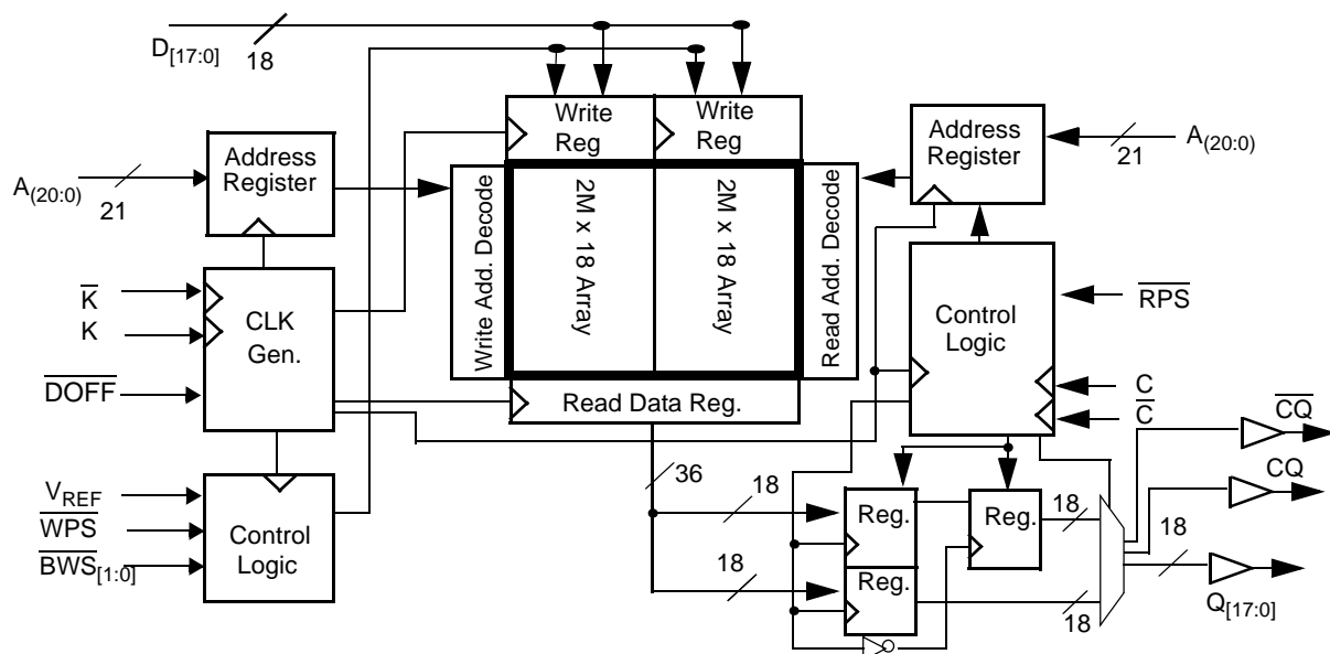
Logic Block Diagram (CY7C1512V18)
