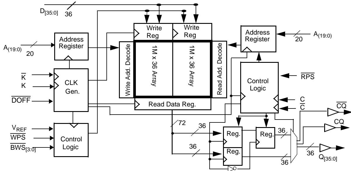
Logic Block Diagram (CY7C1514V18)
