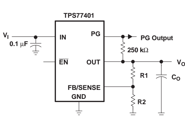
Figure 24. TPS77401 Adjustable LDO Regulator Programming
