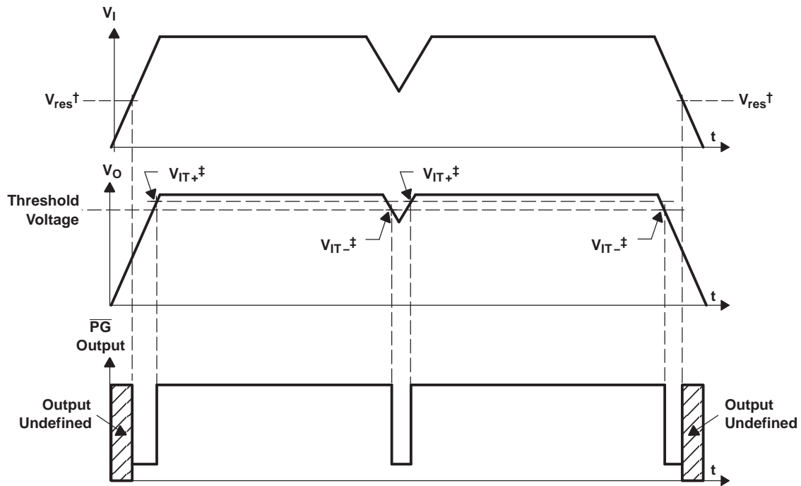
PG TIMING DIAGRAM
