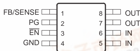
DGK PACKAGE (TOP VIEW)
