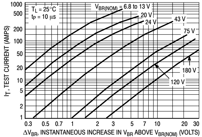
Figure 6. Dynamic Impedance
