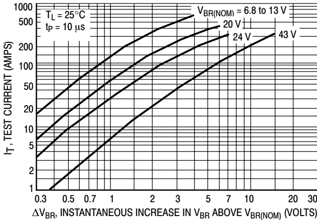
Figure 6. Dynamic Impedance
