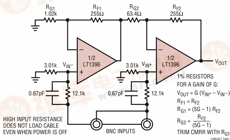
Unity-Gain Video Loop-Through Amplifier
