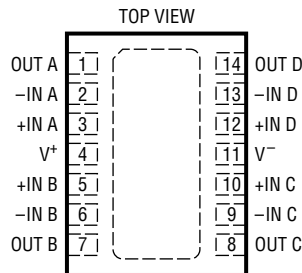
DE14 PACKAGE 14-LEAD (4mm × 3mm) PLASTIC DFN T_{JMAX} = 125^\circ\text{C} , \theta_{JA} = 43^\circ\text{C/W} , \theta_{JC} = 4.3^\circ\text{C/W} EXPOSED PAD (PIN 15) IS V^- MUST BE SOLDERED TO PCB
