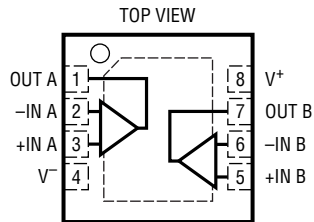
DD PACKAGE 8-LEAD (3mm × 3mm) PLASTIC DFN T_{JMAX} = 125^\circ\text{C} , \theta_{JA} = 160^\circ\text{C/W} (NOTE 3) UNDERSIDE METAL CONNECTED TO V^- (PCB CONNECTION OPTIONAL)
