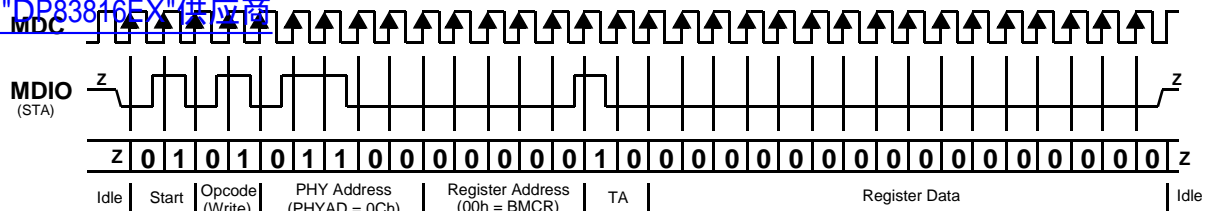
Figure 3-16 Typical MDC/MDIO Write Operation
