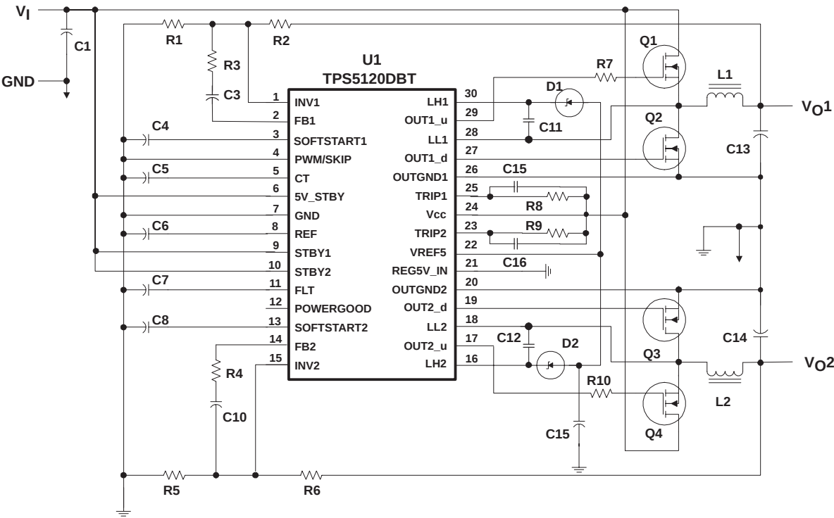
Figure 1. EVM Typical Design
