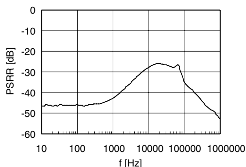
Ripple rejection
