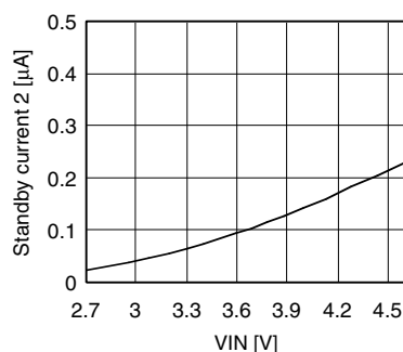
Standby current (VEN = 1.8V)
