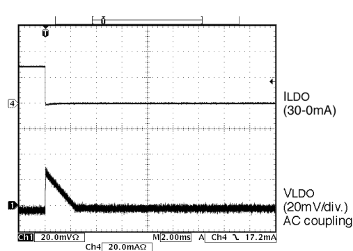
Step response 2
