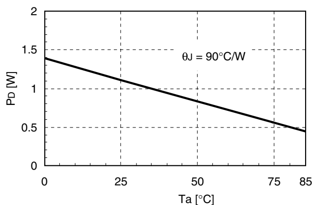
SM8150A power dissipation
