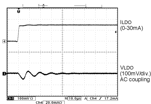
Step response 1
