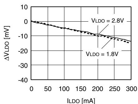
Load regulation
