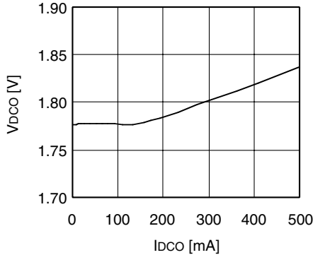
Load regulation
