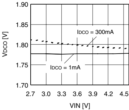
Line regulation
