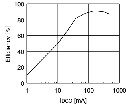
Efficiency – Load current
