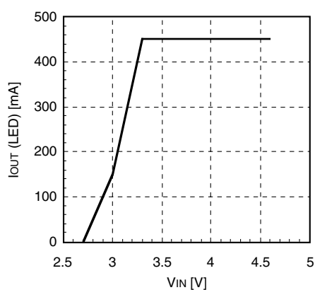
I OUT (LED) vs. V IN
