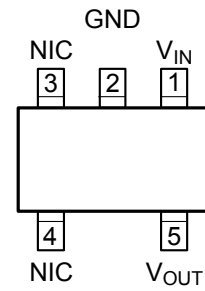
SOT 23-5 (M5) Top View
