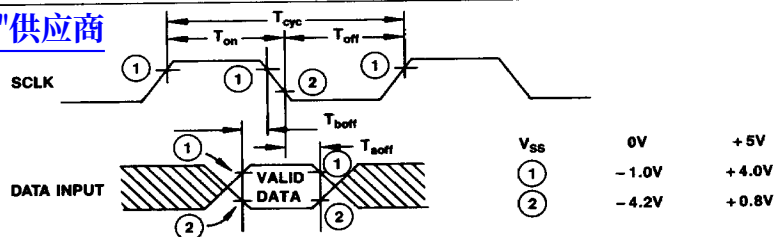
SCLK and Serial Data Timing
