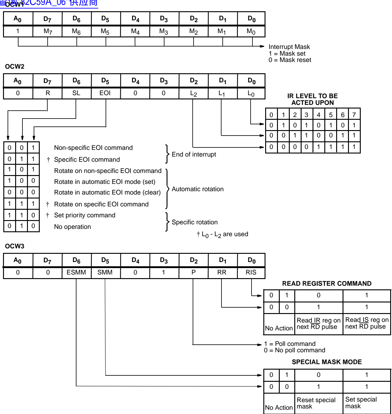
FIGURE 8. 82C59A OPERATION COMMAND WORD FORMAT
