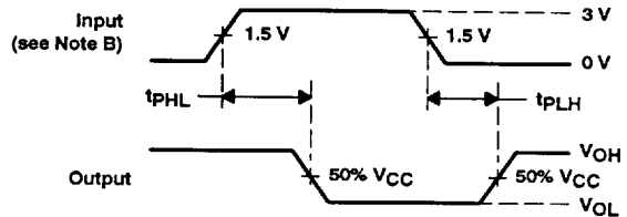
VOLTAGE WAVEFORMS
