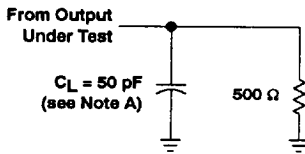
LOAD CIRCUIT
