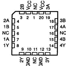
54ACT11000 . . . FK PACKAGE (TOP VIEW)
