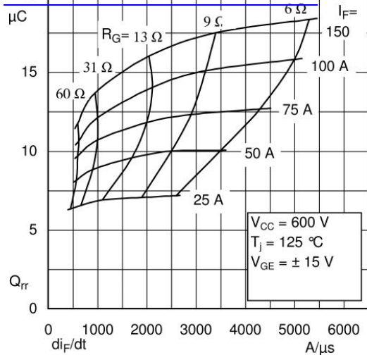
Fig. 13 Typ. CAL diode recovered charge
