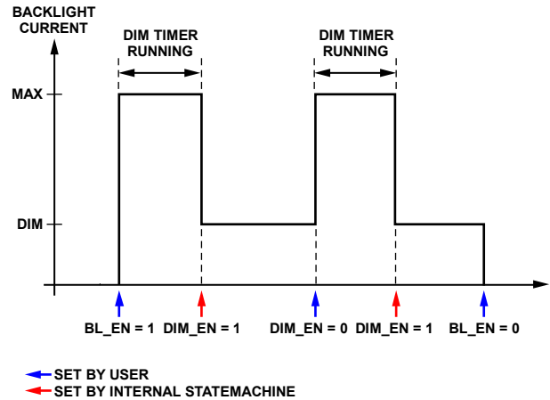
Figure 34. Dim Timer
