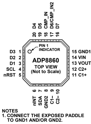
Figure 3. LFCSP Pin Configuration
