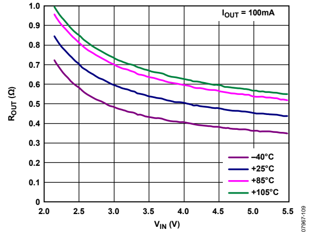
Figure 14. Typical R_{OUT} ( G = 1\times ) vs. V_{IN}
