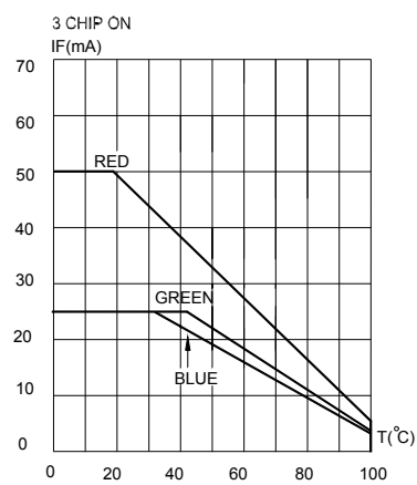
MAXIMUM FORWARD DC CURRENT VS, AMBIENT TEMPERATURE.
