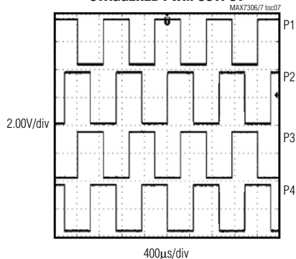
STAGGERED PWM OUTPUT
