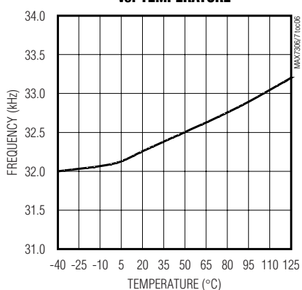
INTERNAL OSCILLATOR vs. TEMPERATURE
