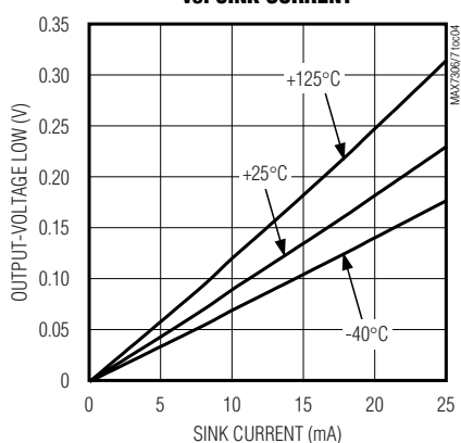
PORT OPEN-DRAIN OUTPUT LOW VOLTAGE vs. SINK CURRENT
