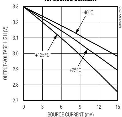
PUSH-PULL OUTPUT HIGH VOLTAGE vs. SOURCE CURRENT
