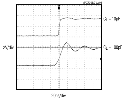
PUSH-PULL OUTPUT RISE TIME
