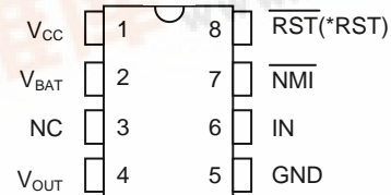
8-Pin DIP (300mil)
