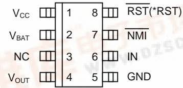
8-Pin SO (150mil)
