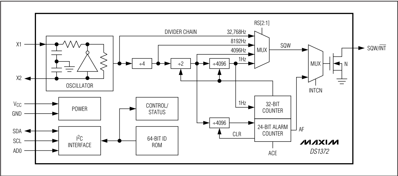
Figure 1. Block Diagram
