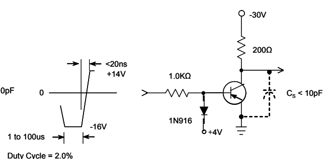
Fig. 2. Turn-Off Time
