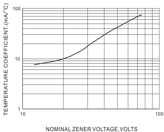
Fig.2 TEMPERATURE COEFFICIENTS
