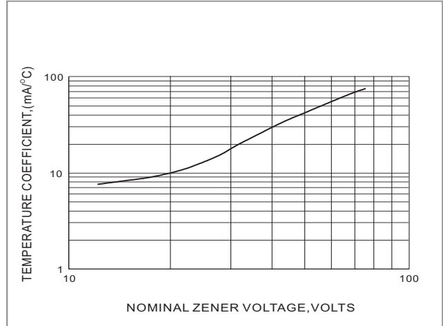
Fig.2 TEMPERATURE COEFFICIENTS
