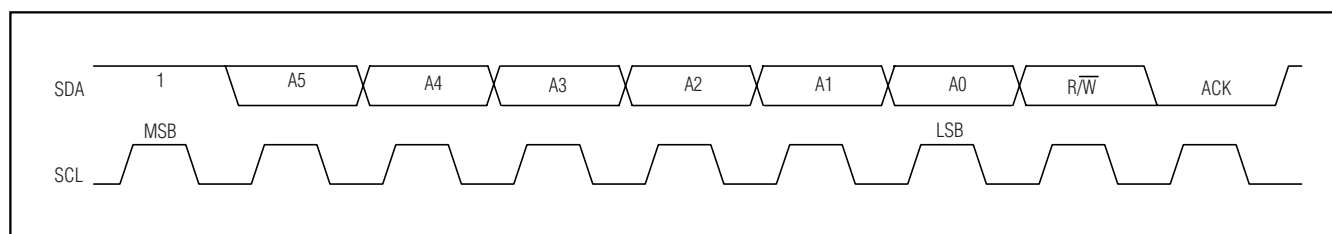
Figure 5. Slave Address
