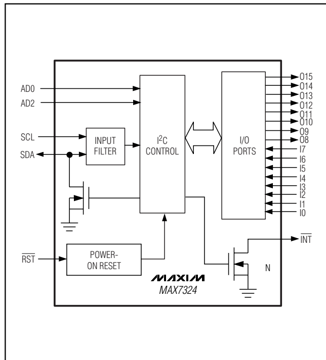
Functional Diagram
