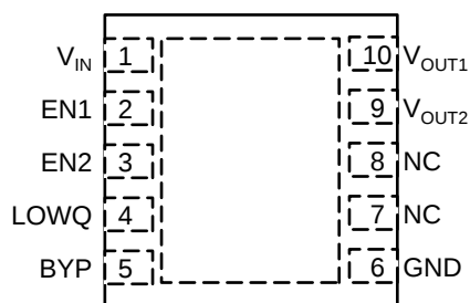
MIC5311-xxBML (3x3)
