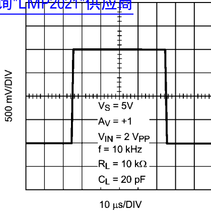
Large Signal Step Response 查询"LMP2021"供应商
