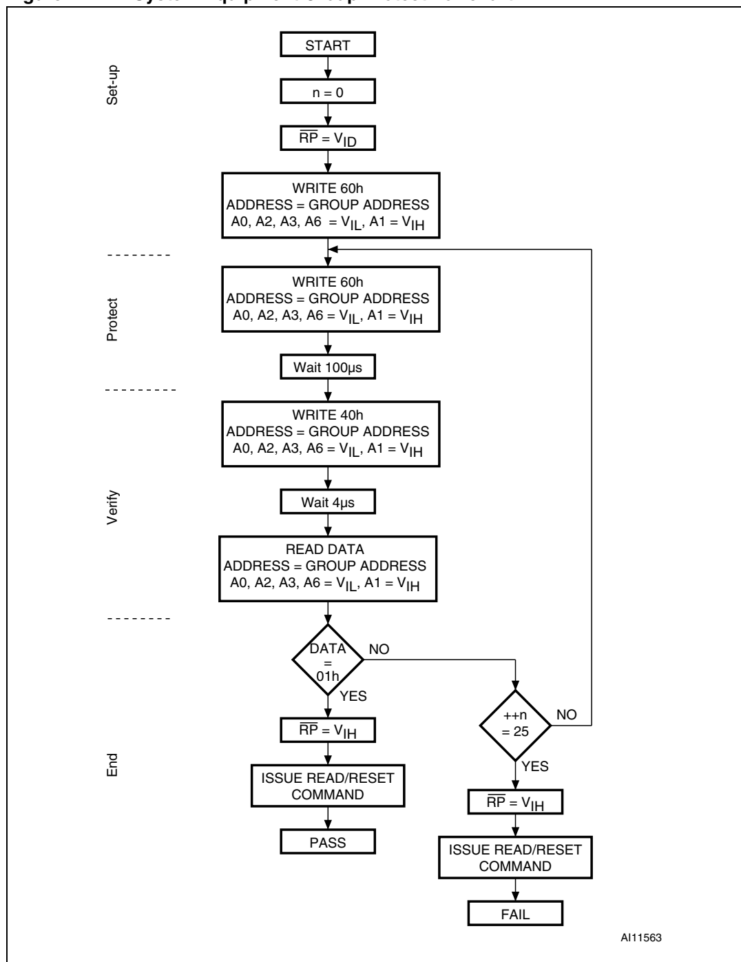
Figure 27. In-System Equipment Group Protect flowchart
