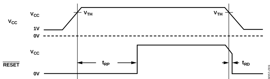
Figure 9. RESET Timing
