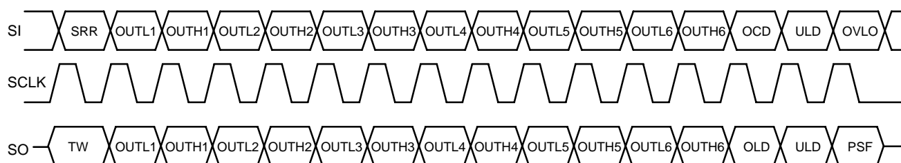
Figure 3. SPI Communication Frame Format
